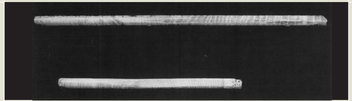
FIG 6 Cores after their cross-sections have been prepared; sapwood is present on the right of the bottom core. It is lighter in colour and contains worm holes
