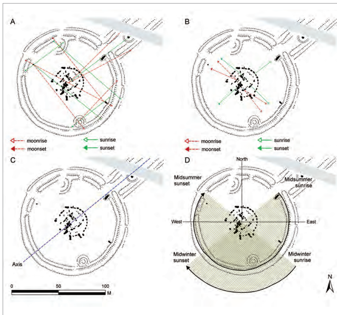
Illustration 80 Stonehenge showing the main astronomical axes and alignments. A: Alignments proposed by Gerald Hawkins for the early phases of Stonehenge and (B) alignments through the central trilithons. C: The main northeast-southwest axis projected onto Phase 3 of the monument. D: Schematic representation of the main solar movements in relation to Phase 3 of the monument. [A and B based on Hawkins 1966a, figures 11 and 12; C after Cleal et al. 1995, figure 79; D after Atkinson 1987, 11.]
