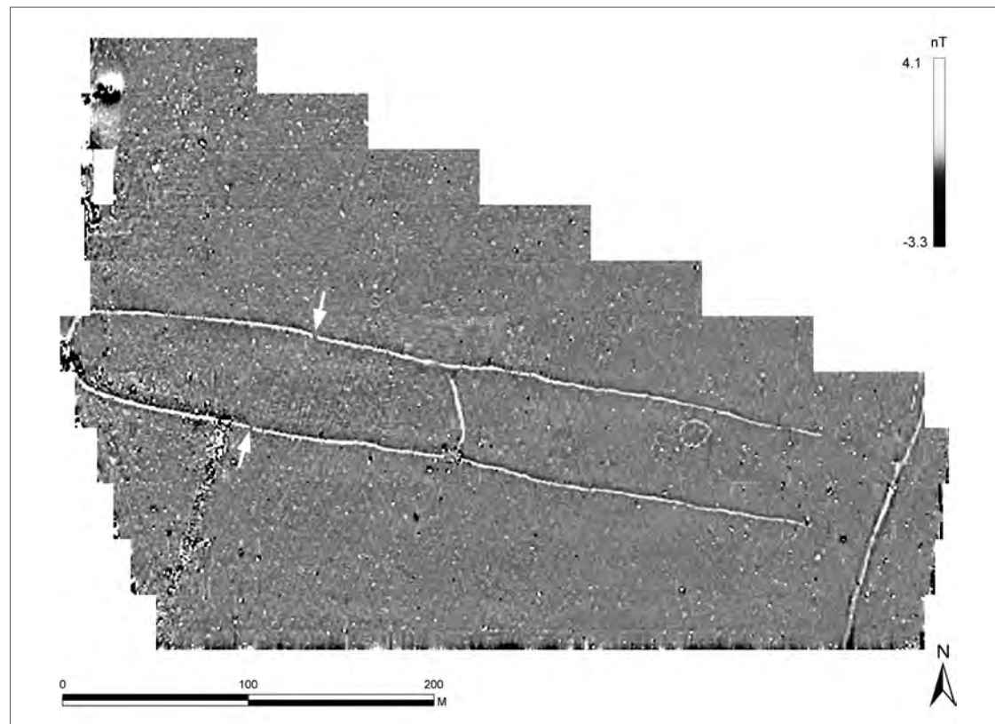
Illustration 10 Plot of the results from a geophysical survey of the Lesser Cursus in 1993. [Survey by Alastair Bartlett for English Heritage.]
