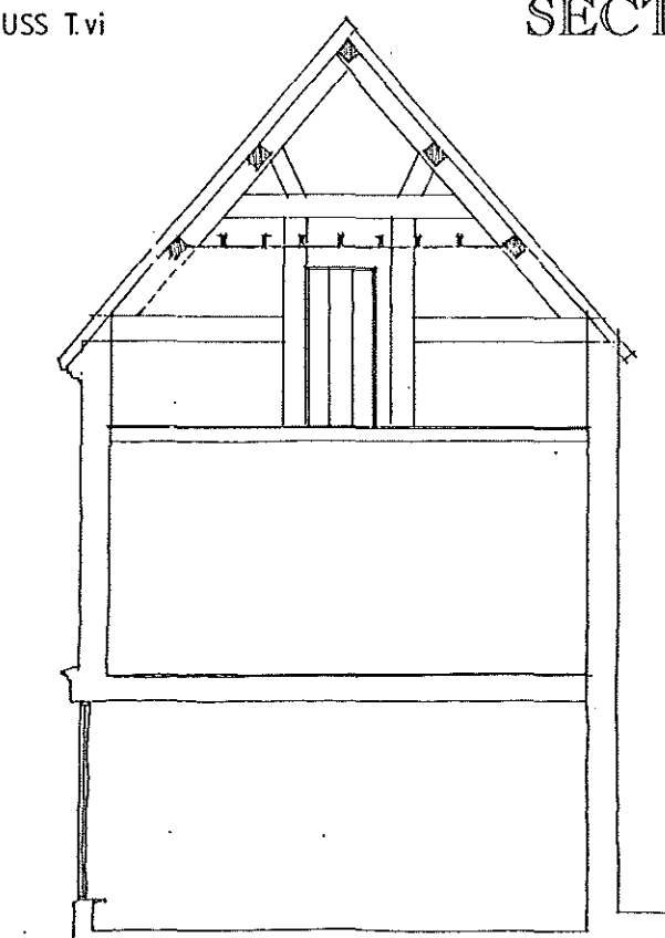
SECTION J-J TRUSS T.ix
