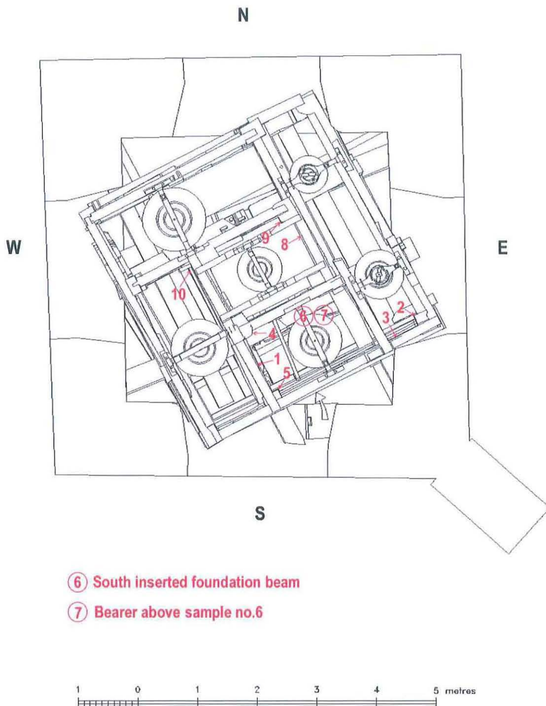
Figure 4: Plan of the bellframe showing the locations of the samples taken for dendrochronology, English Heritage, July 2003
