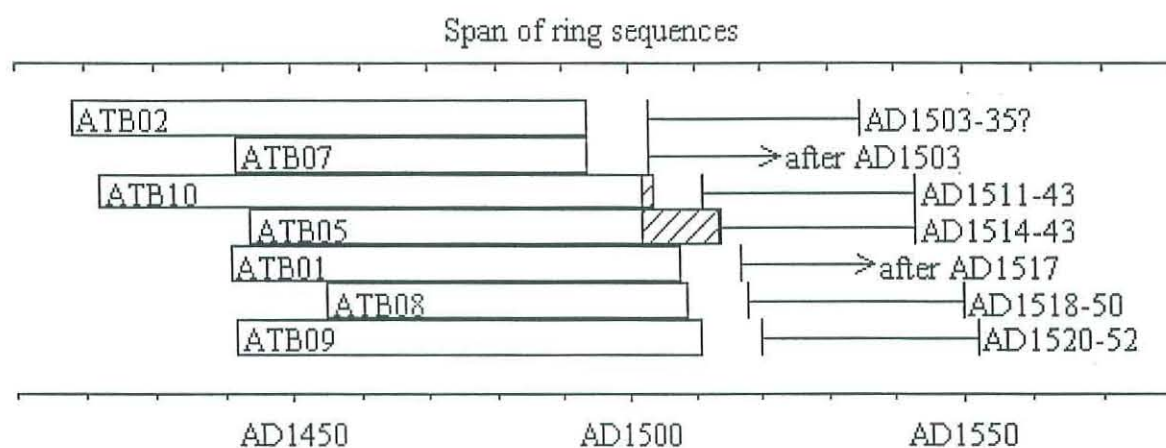
Figure 5: Bar diagram showing the relative positions of overlap of the dated timbers from the bellframe at St Mary's Church, Attleborough, Norfolk, along with their interpreted felling dates
