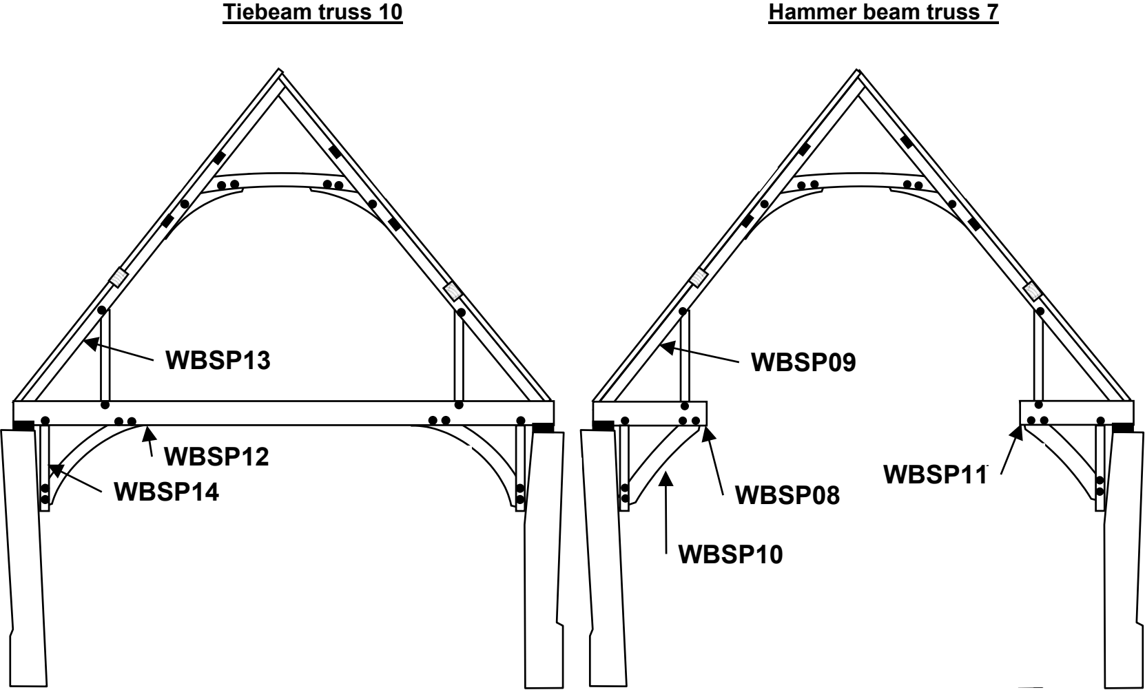
Figure 7: Section of trusses T7 and T10 at Waxham Great Barn, showing the multiple cores sampled from these trusses (adapted from Heywood).
