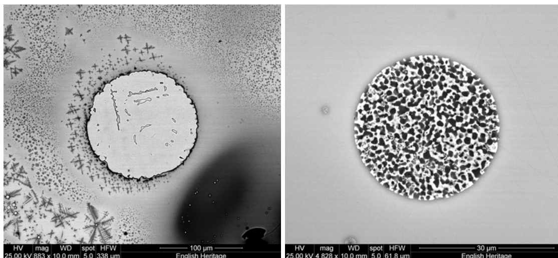
Figure 2: Two BSE images of metallic droplets 2.1 (left) and 4.1 (right).
