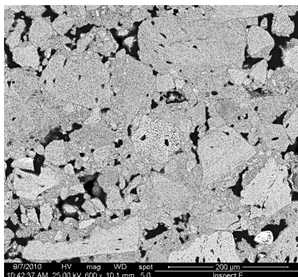
Figure 1. SEM micrographs of cupel GEC00(24). The top image shows the impregnated cupel with the light-coloured, inter-granular areas rich in lead. The scale bar is 500µm. The bottom image shows the unimpregnated base area, with calcined bone grains visible in a fine bone-ash matrix. The scale bar is 200µm.
