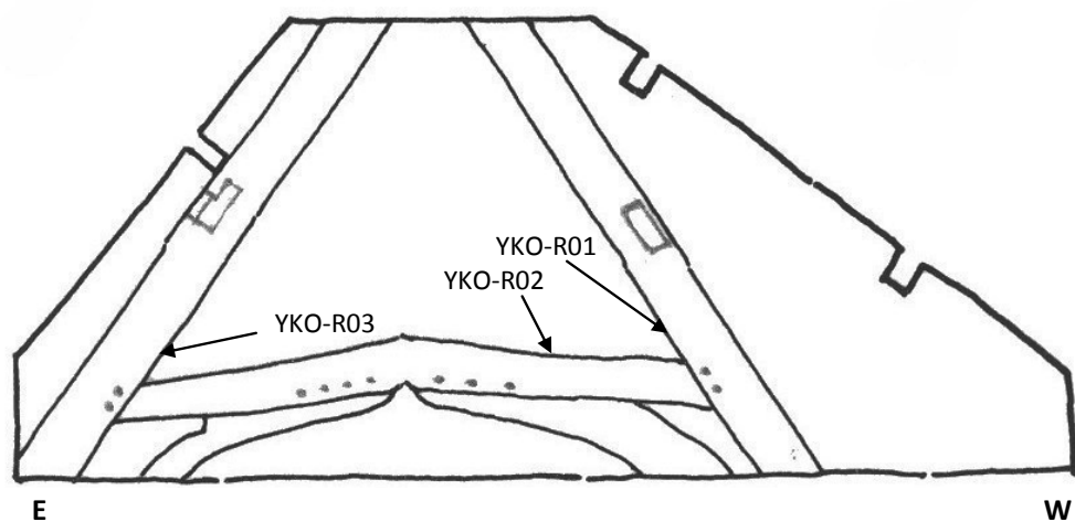
Figure 11: North face of truss E showing the sample locations
