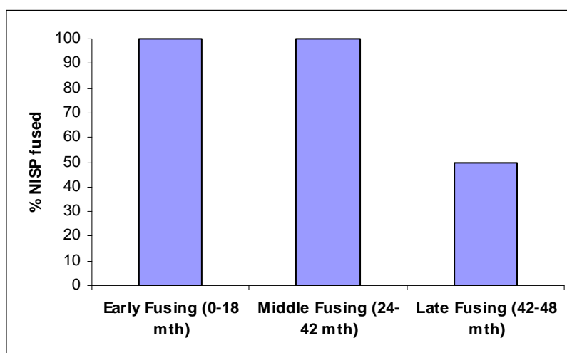
Figure 6: Cattle epiphyseal fusion data for Phase 4b
