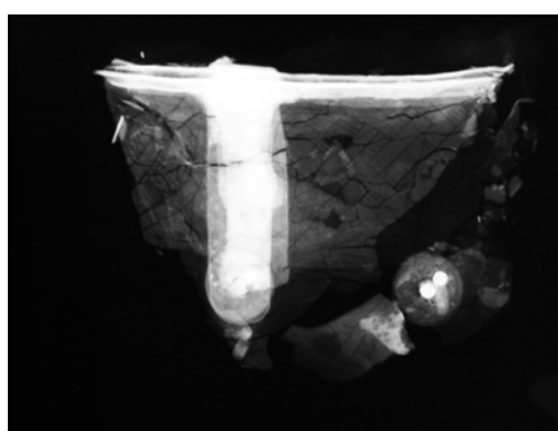
Figure 35: SF 889 X-radiograph illustrates the layers of copper alloy forming the rim mount.
