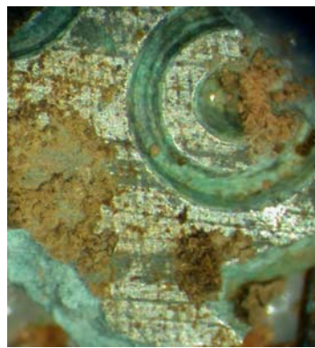
Figure 55: SF 793 Tinned surface.
