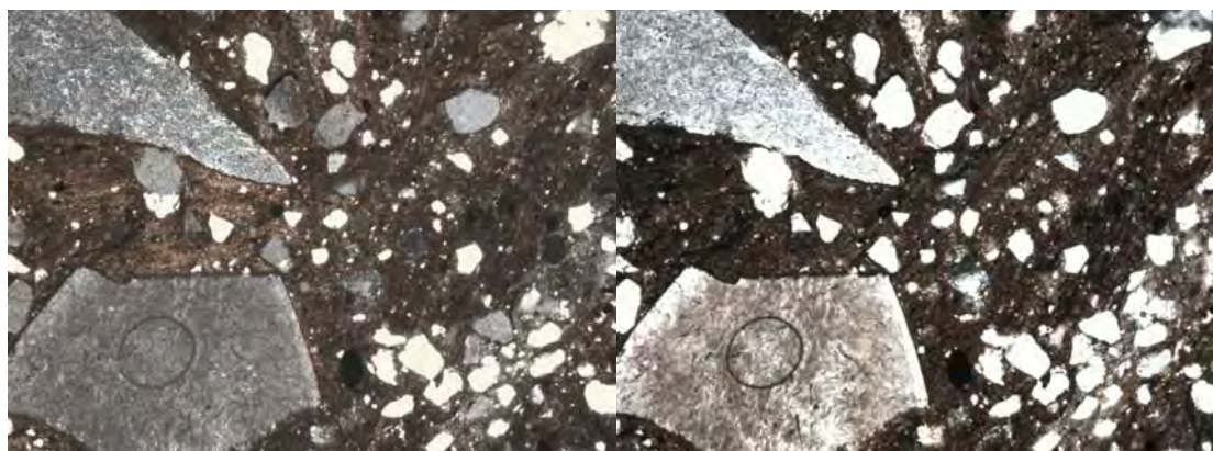
Figure 4: Thin section photomicrographs of Fabric 2, Sample NI61 (Peterborough Ware). Left image is taken in XPL and right image is taken in PPL. Showing angular flint inclusions (grey) in a silt to sand-sized quartz matrix. Width of image is 2.8mm.
