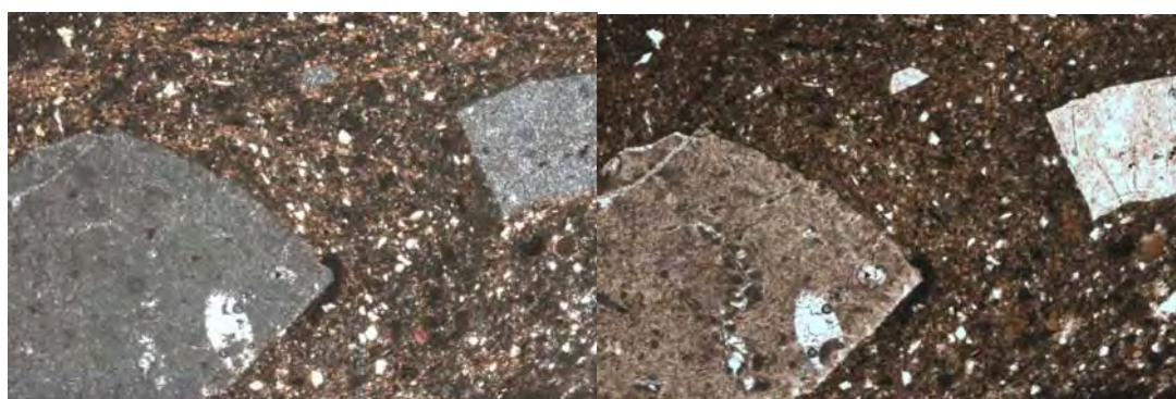
Figure 3: Thin section photomicrographs of Fabric 1, Sample NI60 (Windmill Hill Ware). Left image is taken in XPL and right image is taken in PPL. Showing angular flint inclusions (grey) in a silt and very fine sand-sized quartz matrix, similar to the Silbury Hill clay-with-flints (Figures 1 and 2). Width of image is 2.8mm.
