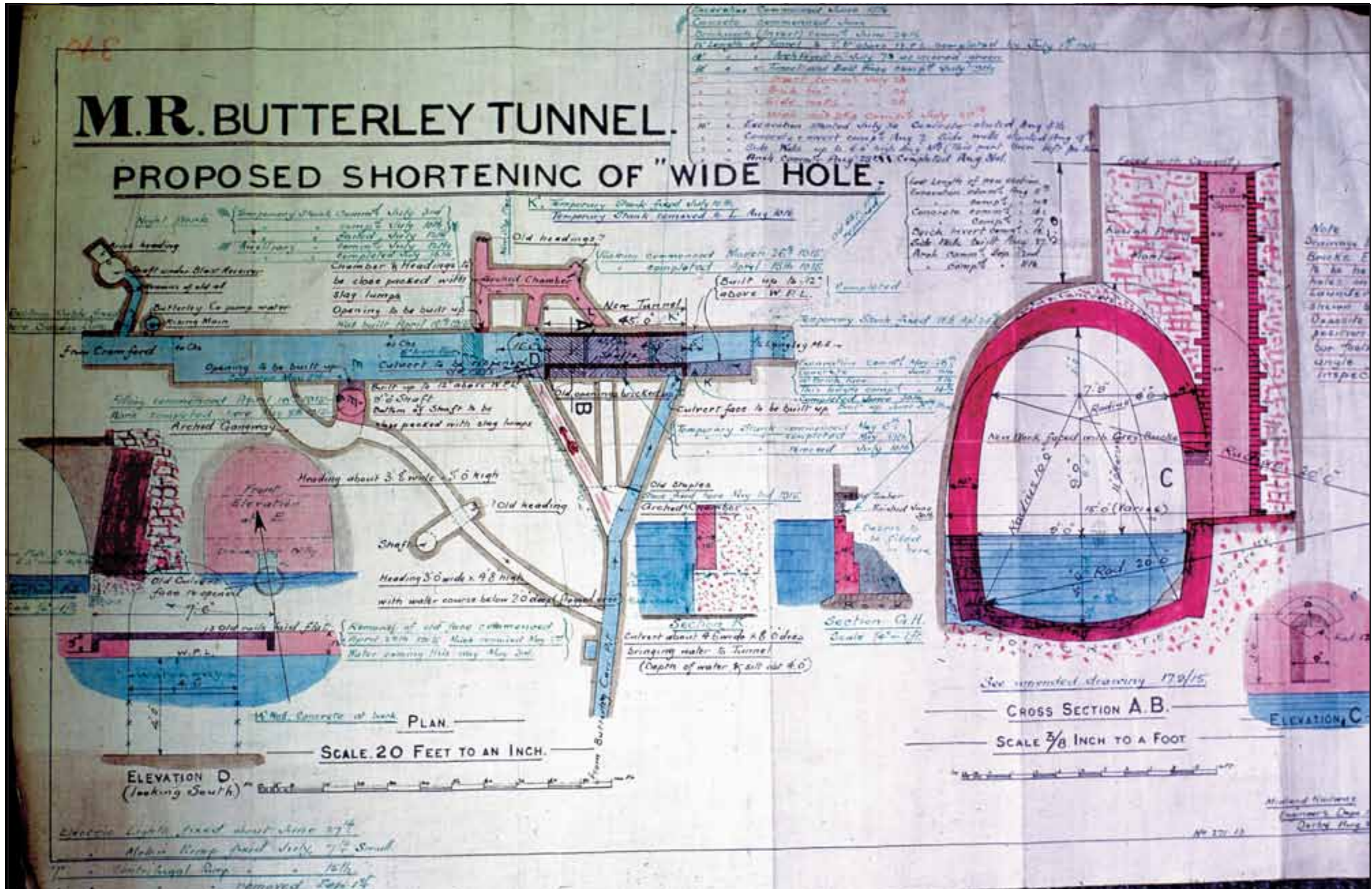
Figure 9: Midland Railway Plan showing the 'proposed shortening of the wide hole', with annotations from 1915 detailing progress of the work
