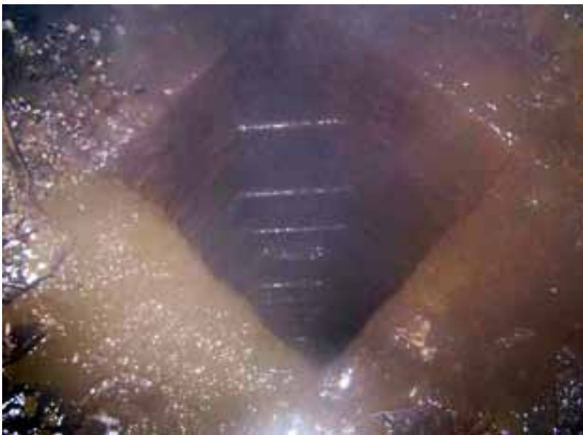
Figure 16: Western loading shaft looking down through the narrowed square opening (after Cordon 2006, image 85), © Tina Cordon, reproduced with permissions
