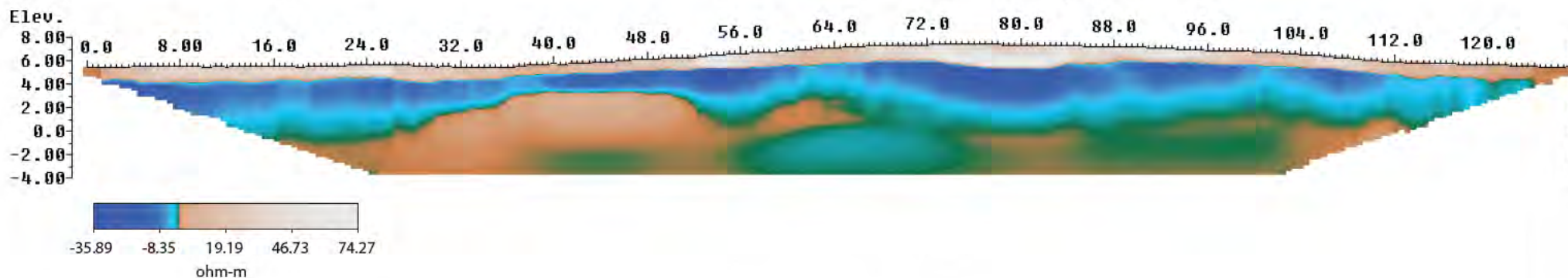
(B) Equal area colourscale plot of subsurface model after enhancement with a vertical ID 4m Gaussian high-pass filter
