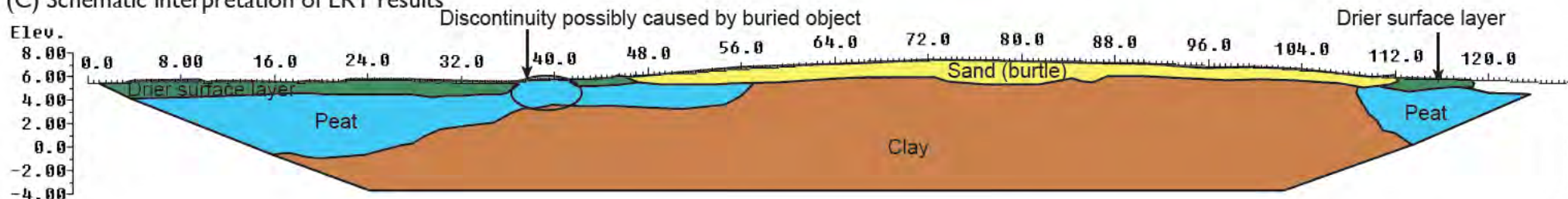
(C) Schematic interpretation of ERT results
