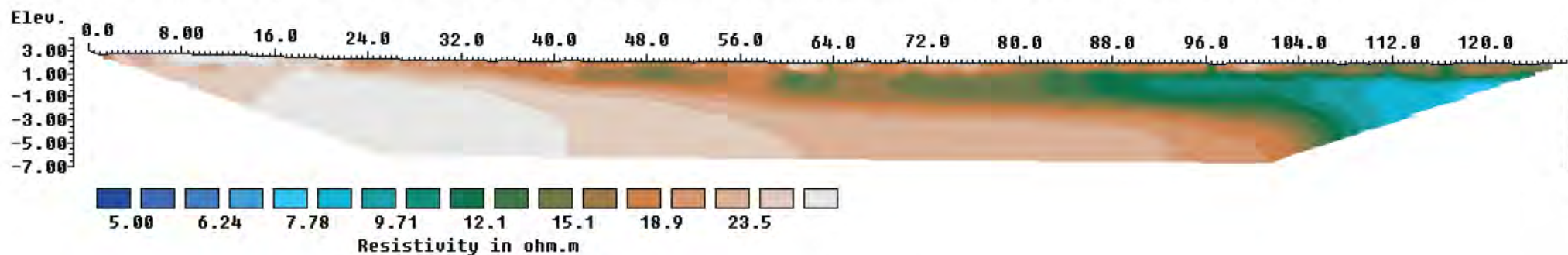
(A) Log linear colourscale plot of subsurface model after inversion (absolute error between model and field measurements = 2.5%)
