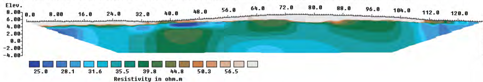
(A) Log linear colourscale plot of subsurface model after inversion (absolute error between model and field measurements = 2.0%)
