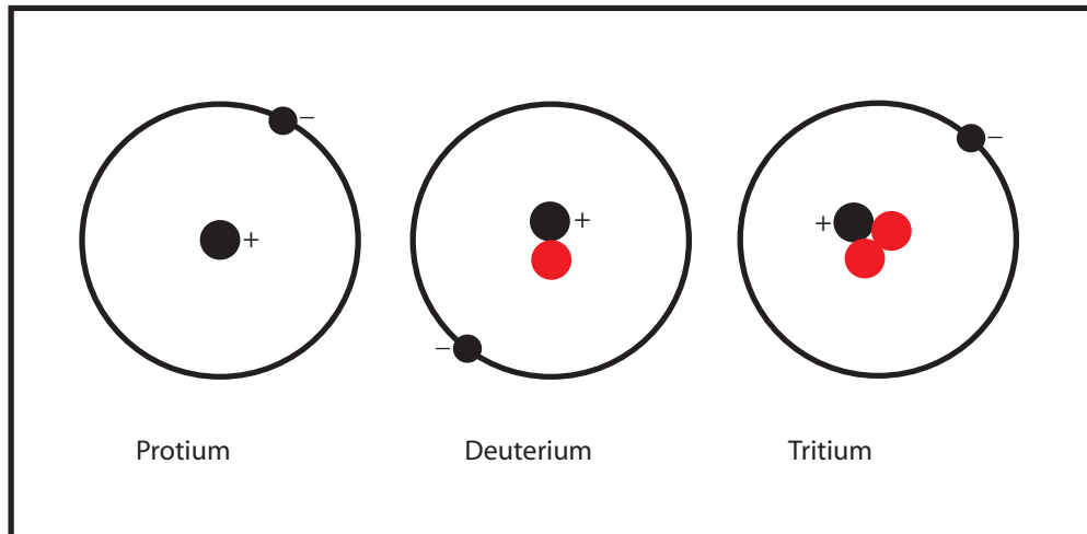
Figure 22 Nuclear isotopes
