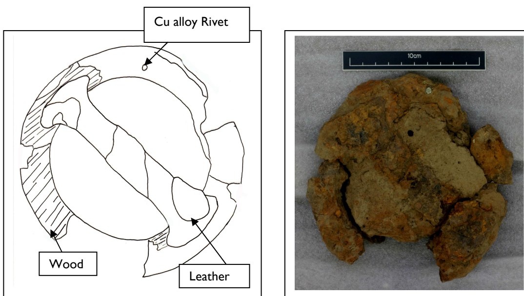
Figure 21. Drawing and photo of the underside of the shield boss with the hand grip
