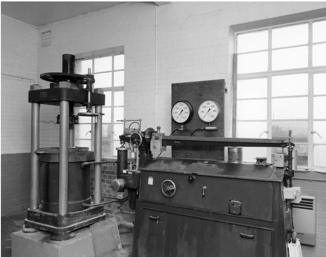
Figure 29: Office, Casting Workshop and Laboratory S5, press by A Macklow Smith Ltd, London and a Beacham high pressure oil pump. These were used for stress testing various materials. (c) English Heritage BB99/15969
