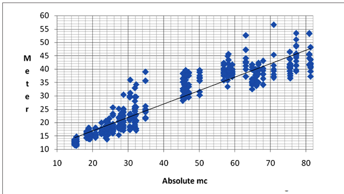
Figure 10: High Bickington Church. Moisture meter readings against actual moisture content of timber dowels. © Ridout Associates
