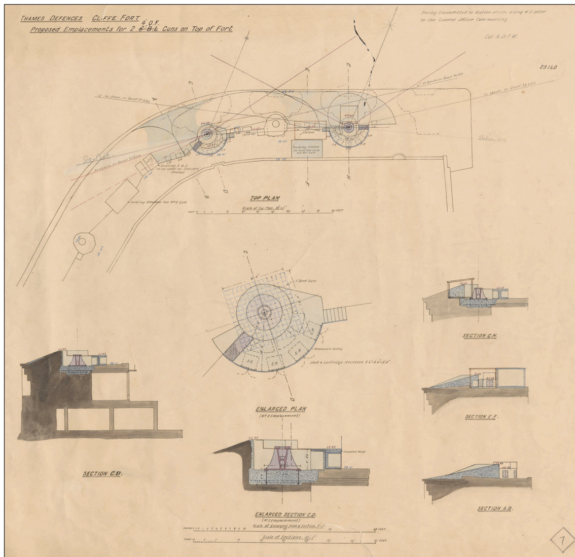
Figure 50: Plan for the proposed emplacements for two 6-inch BL (struck out and replaced with two 4-inch QF) guns on the roof of Cliffe Fort dated 9 May 1913. (TNA: WO78/4963)
