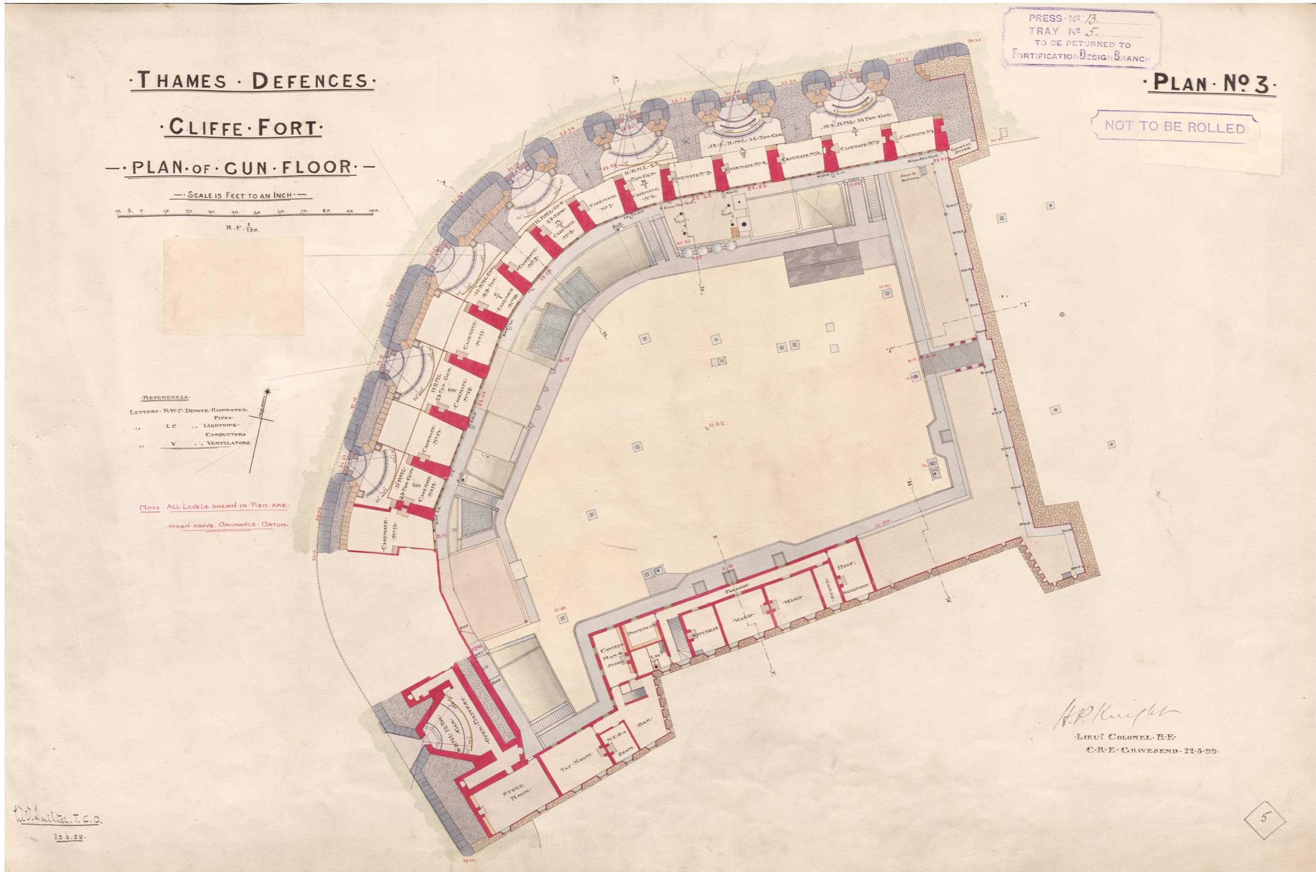
Appendix Figure 2: Thames Defences: Cliffe Fort: Plan of Gun Floor 1899 ©The National Archives: WO78/4963
