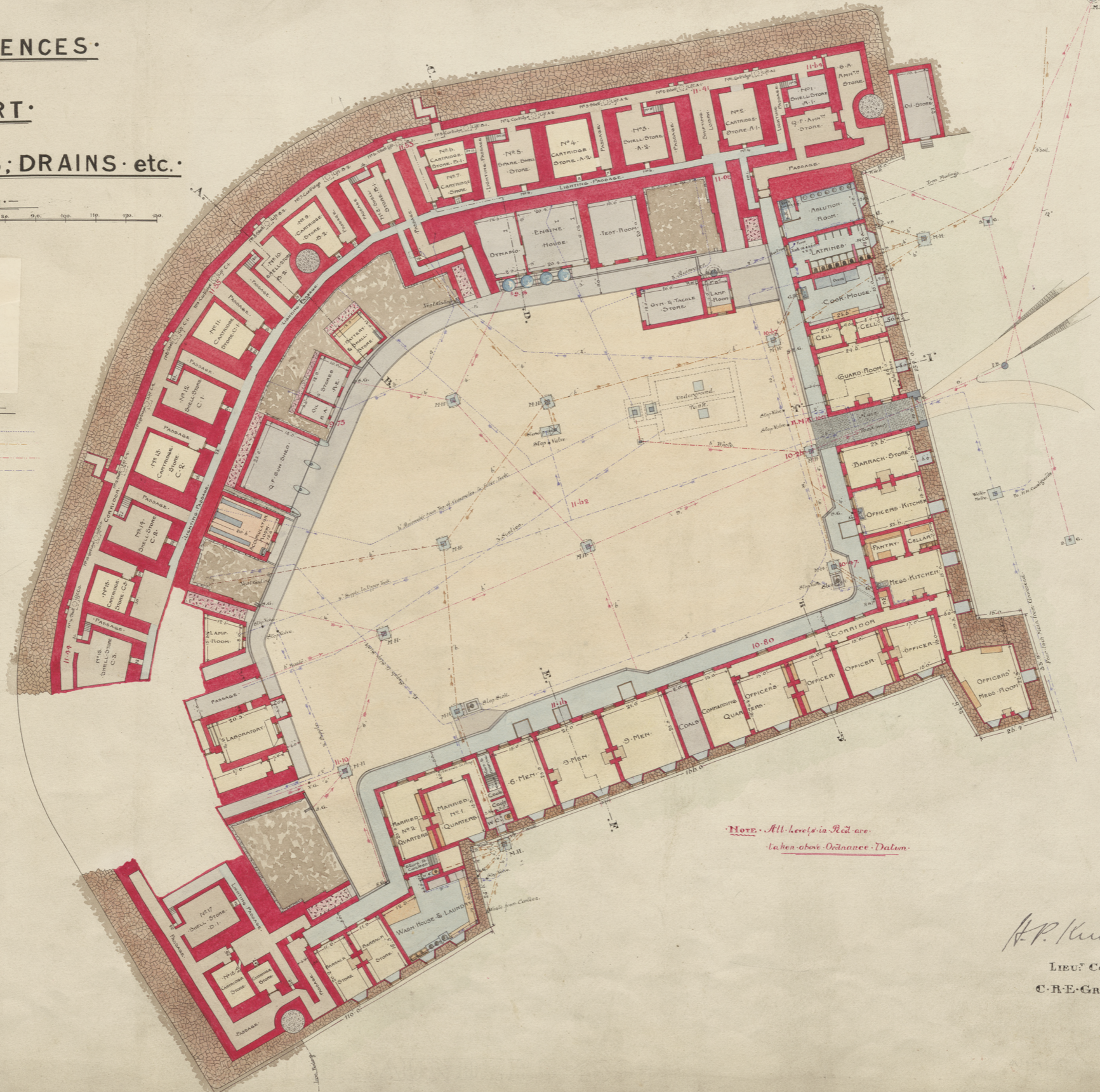
Appendix Figure 1: Thames Defences: Cliffe Fort: Plan of Magazines, Drains etc 1899 ©The National Archives: WO78/4963
