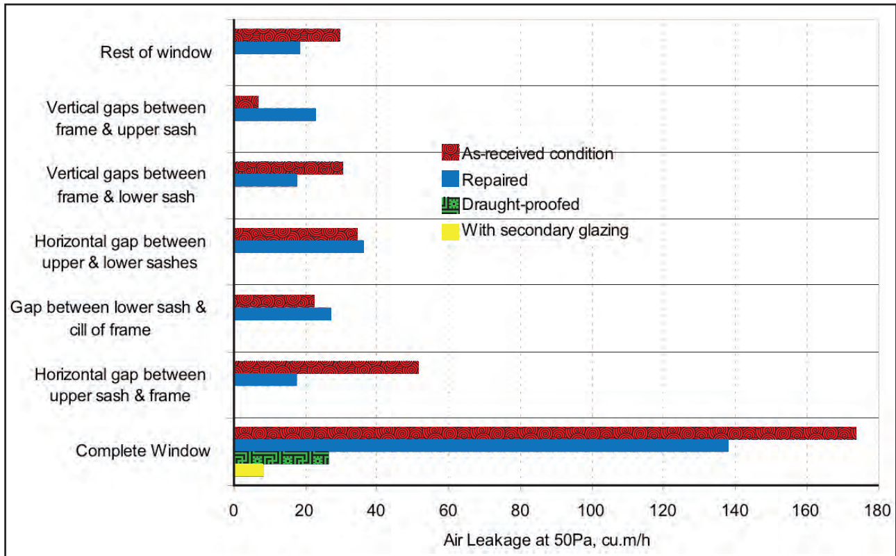
Above: Comparison of the main air leakage paths before and after repair of window
