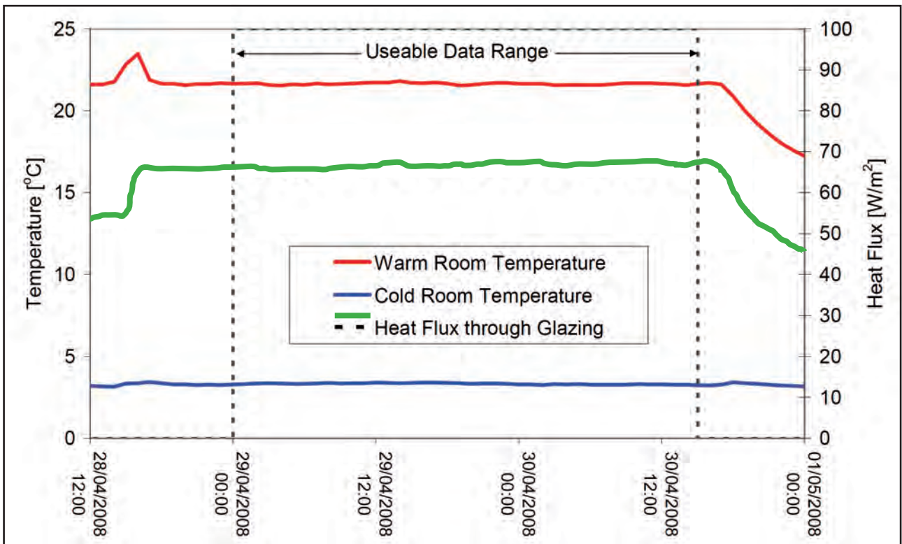
Above: Example of test, showing warm and cold room temperatures and heat flux through glazing.
