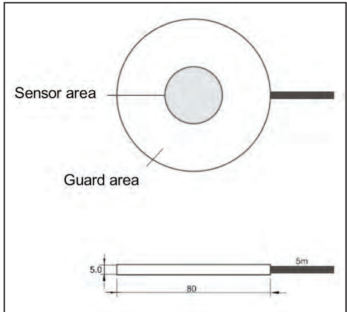
Left: Heat flux sensor positions on glazing; above sensor dimensions
