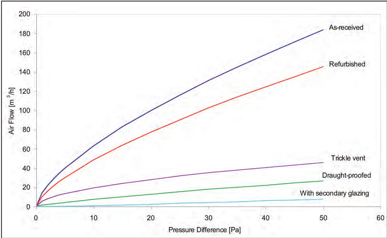
Above: Air leakage characteristics of the window in as-received condition, after repair, after draught-proofing and following installation of secondary glazing. The air leakage characteristic of a trickle vent is included for comparison.
