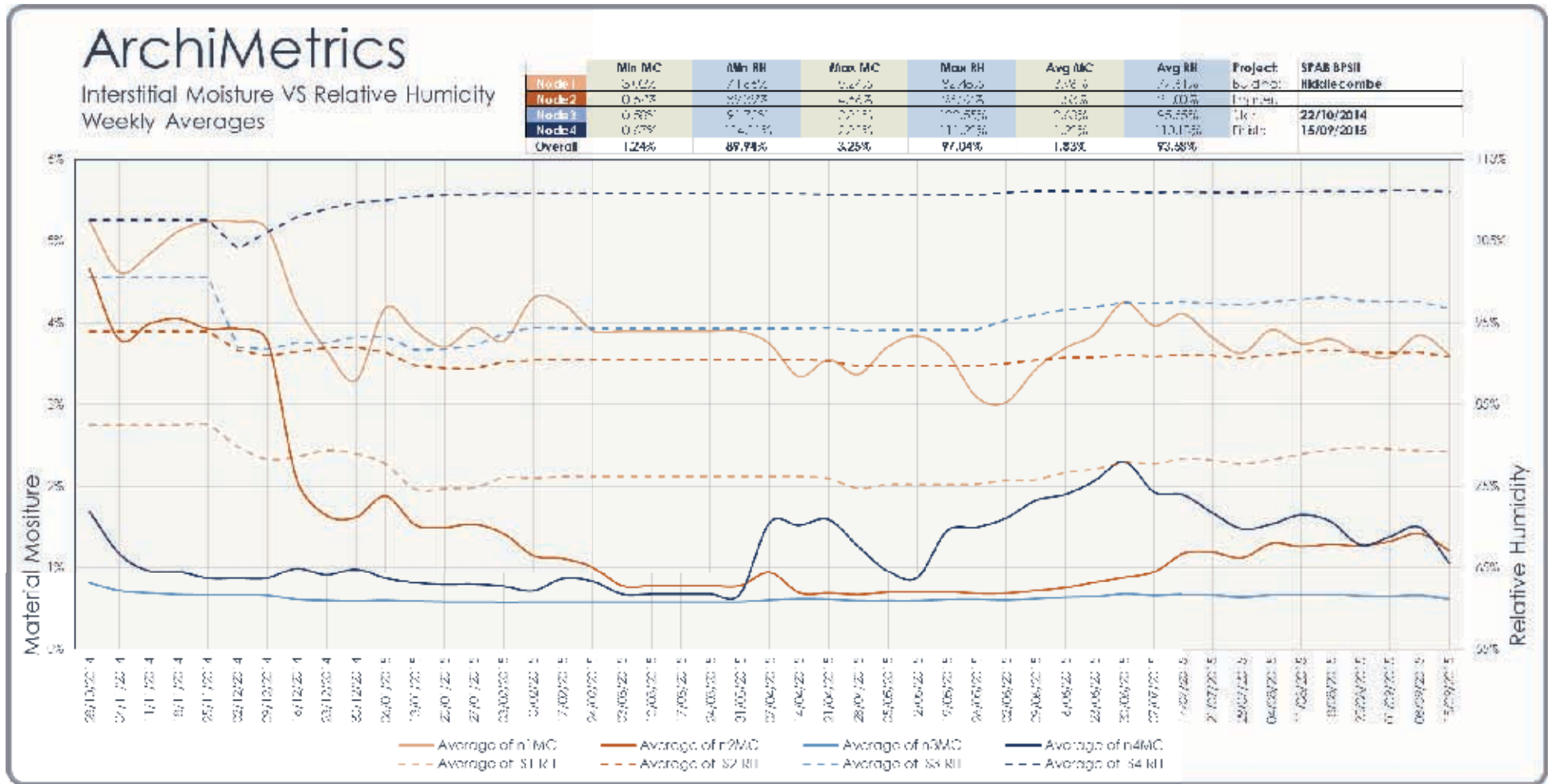
Figure 45: %MC and %RH comparison, The Firs, Riddlecombe, 2014 - 2015.
