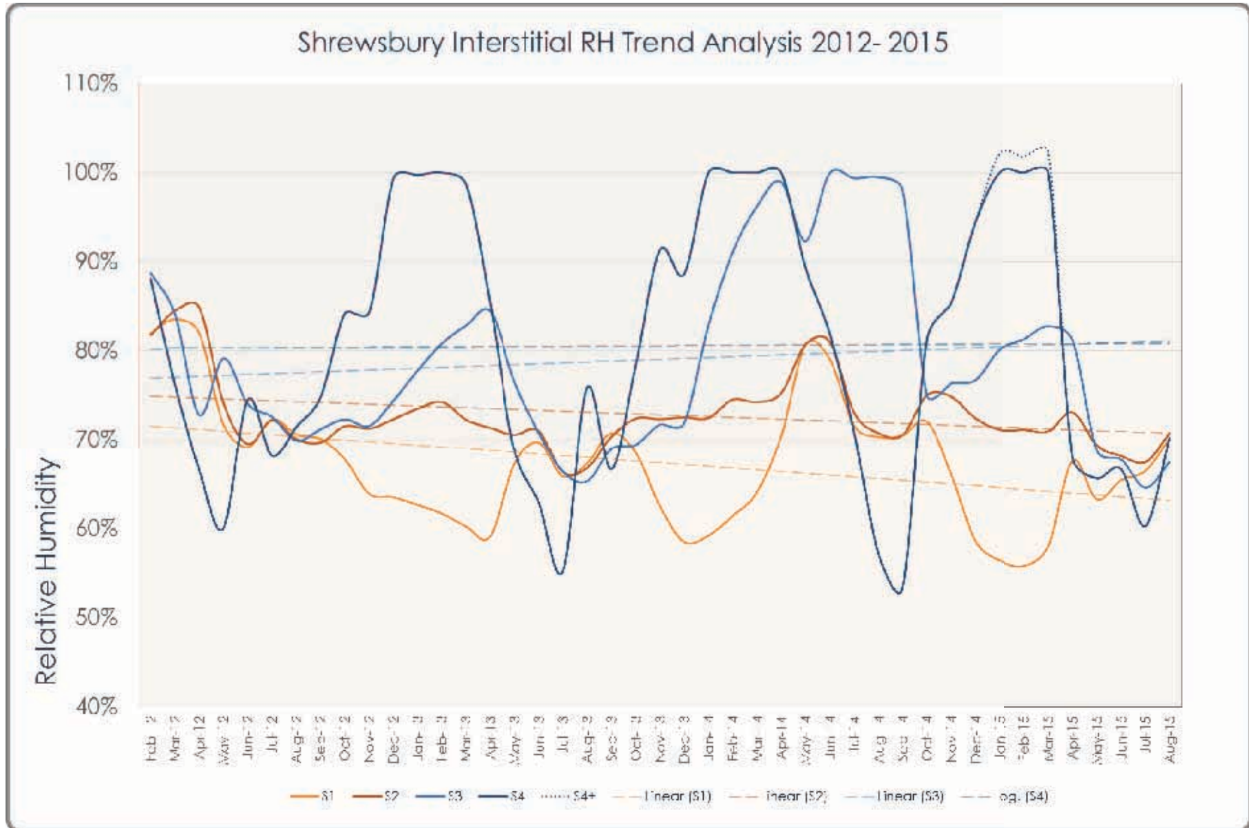
Figure 36: Relative Humidity Trends over time, Shrewsbury 2012 - 2015.
