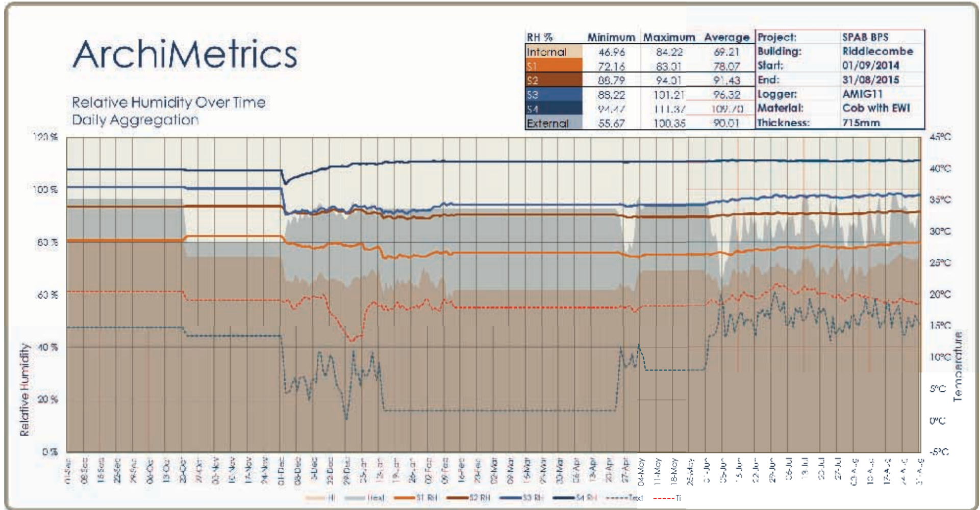
Figure 28: Relative Humidity over time, The Firs, Riddlecombe 2014 - 2015.
