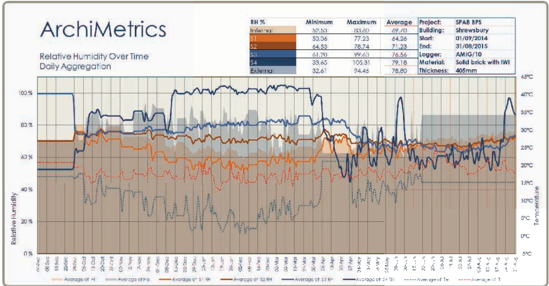
Figure 5: Relative Humidity over time, Abbeyforegate, Shrewsbury 2014 - 2015.
