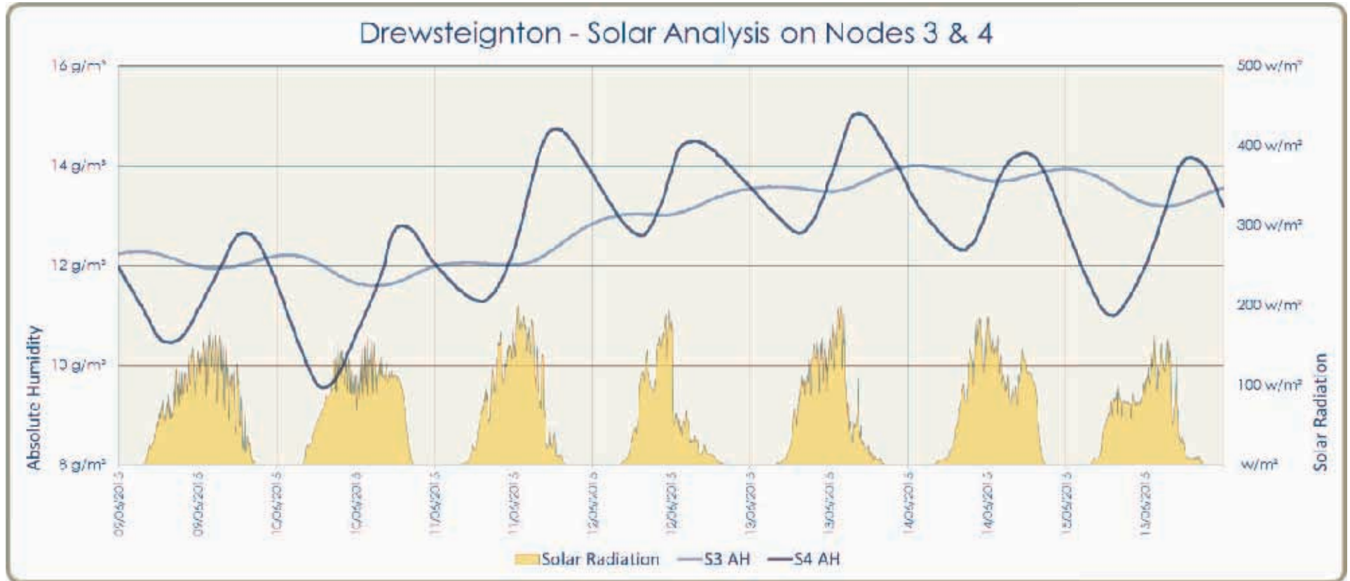
Figure 20: Solar Analysis sensors 3 and 4, Drewsteignton, June 2015.
