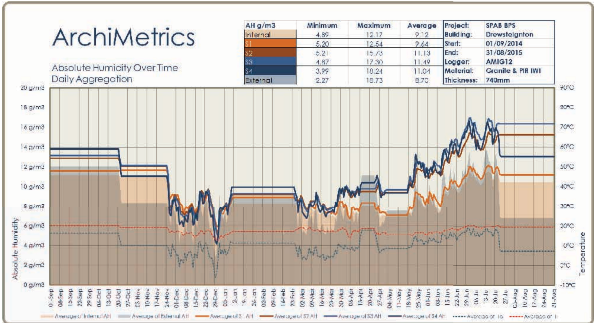
Figure 19: Absolute Humidity over time, Mill House, Drewsteignton 2014 - 2015.
