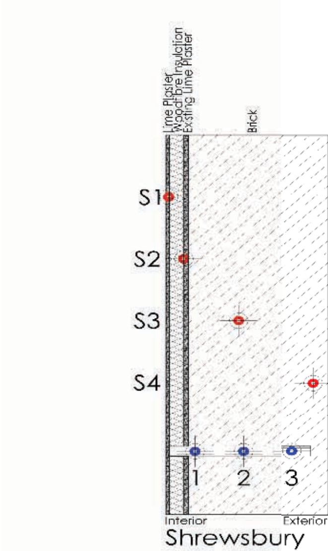
Figure 4. Position of wall sensors through section, Shrewsbury □ red IHGM, blue Material Moisture
