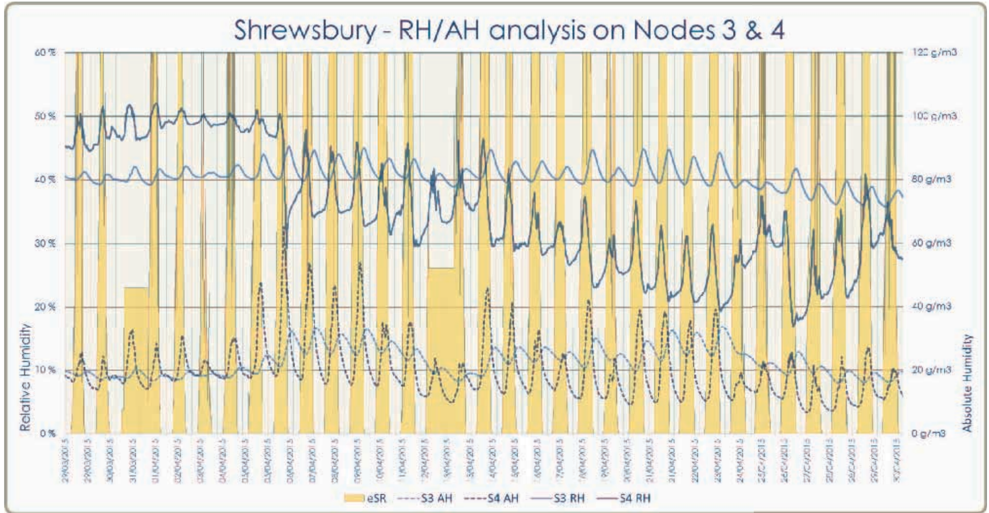
Figure 9: AH and RH Solar Analysis sensors 3 & 4 over time, Abbeyforegate, Shrewsbury 2014 - 2015. 2
