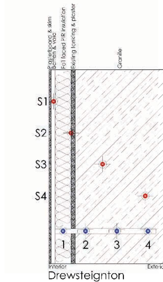
Figure 17. Position of wall sensors through section, Drewsteignton □ red IHGM, blue Material Moisture
