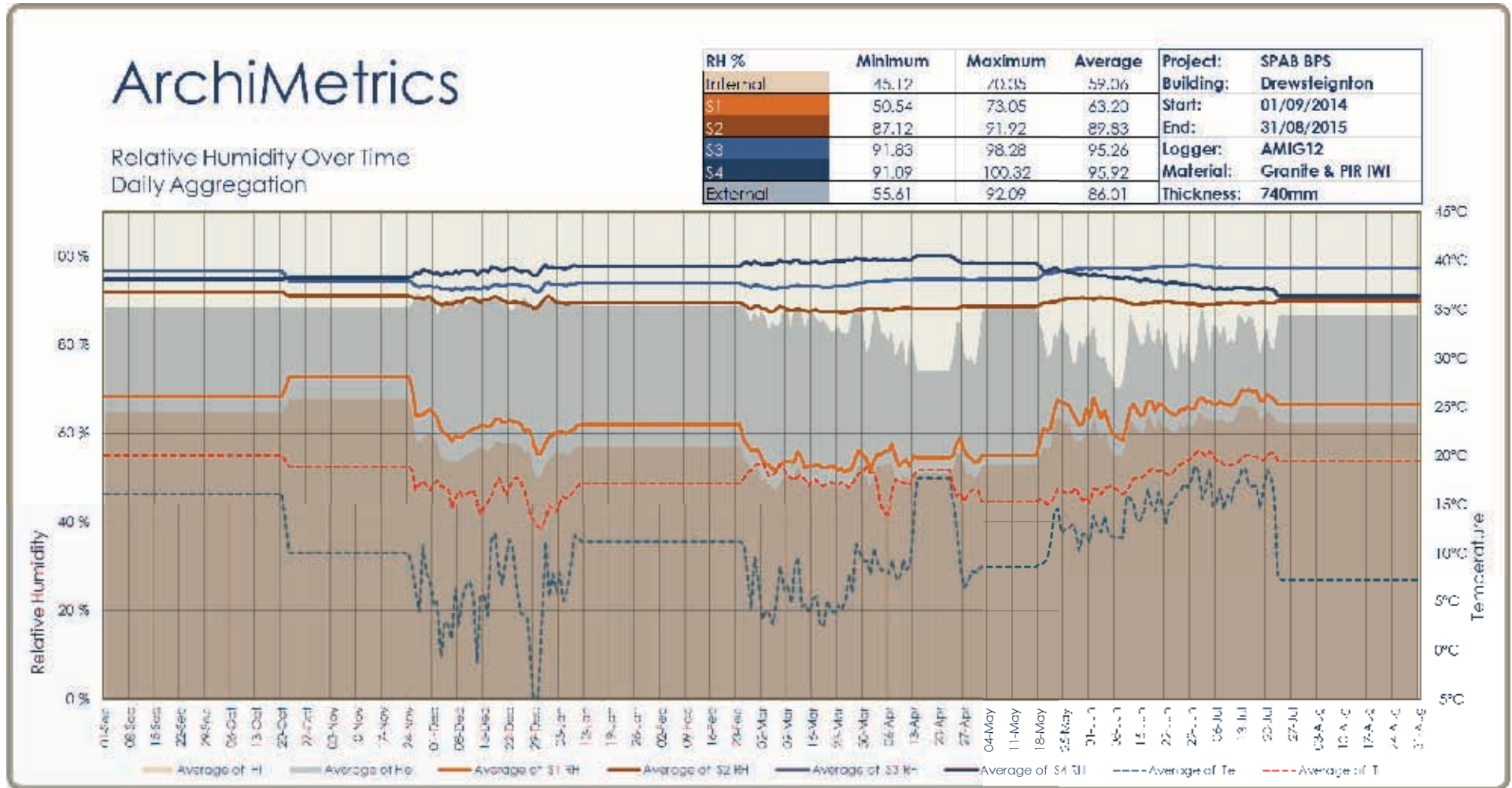
Figure 18: Relative Humidity over time, Mill House, Drewsteignton, 2014-2015.
