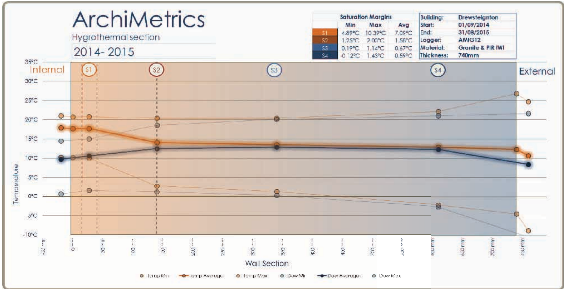
Figure 22. Hygrothermal Section, Mill House, Drewsteignton, 2014 □ 2015 (capped).
