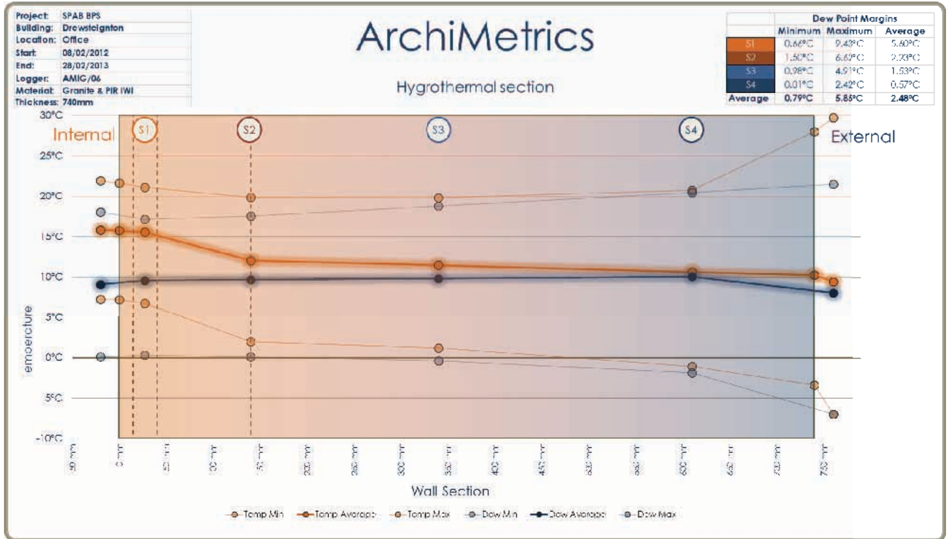
Figure 24. Hygrothermal Section, Mill House, Drewsteignton, 2012 - 2013.
