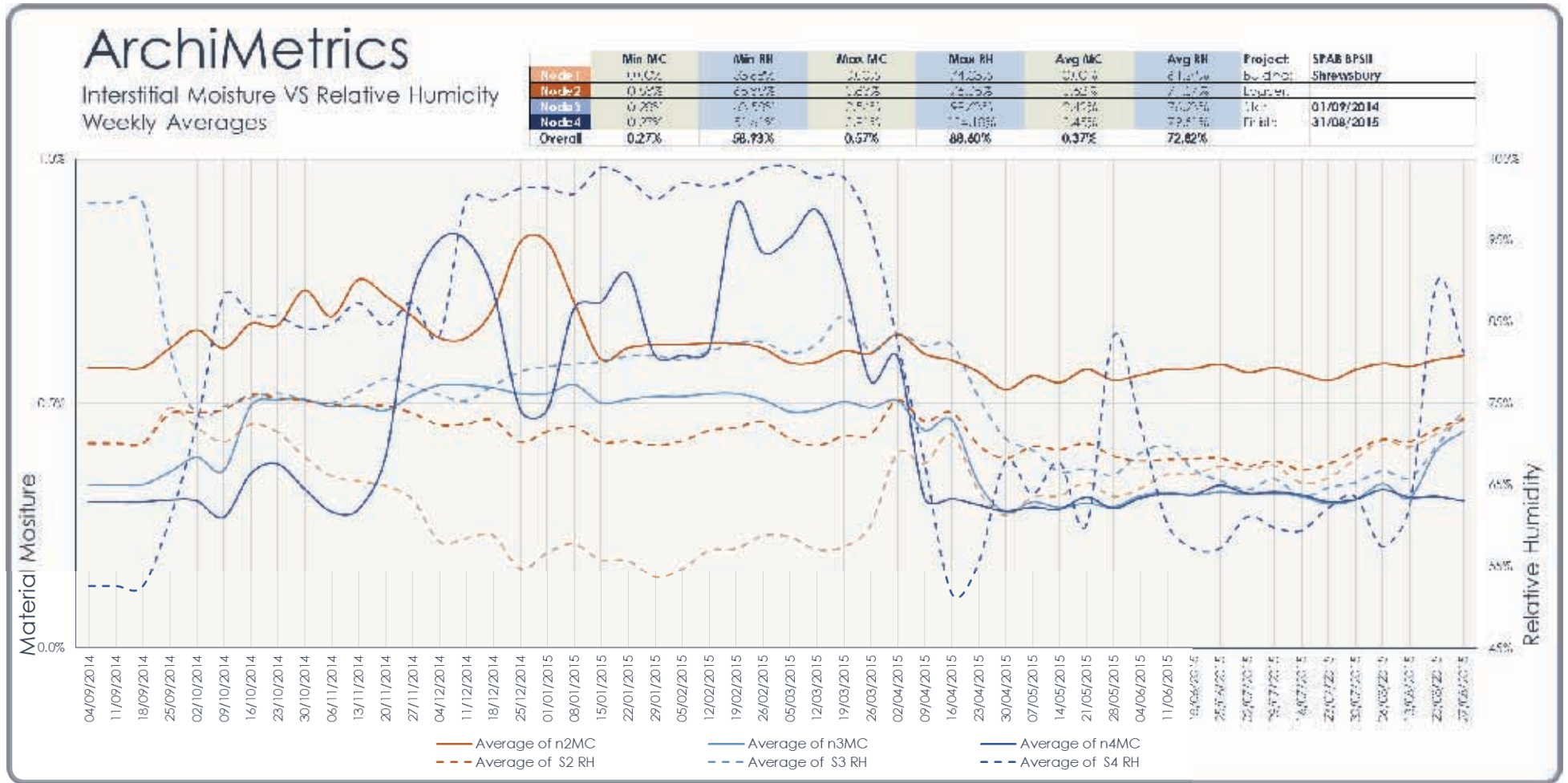
Figure 43: %MC and %RH comparison, Abbeyforegate, Shrewsbury 2014 - 2015.
