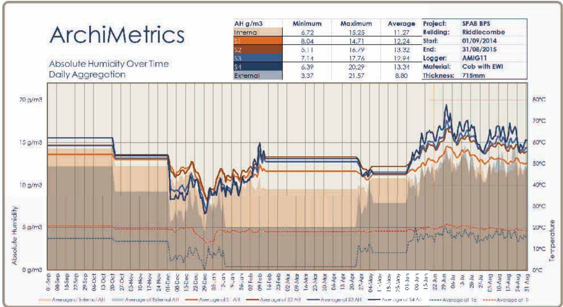
Figure 30: Absolute Humidity over time, The Firs, Riddlecombe, 2014 - 2015.
