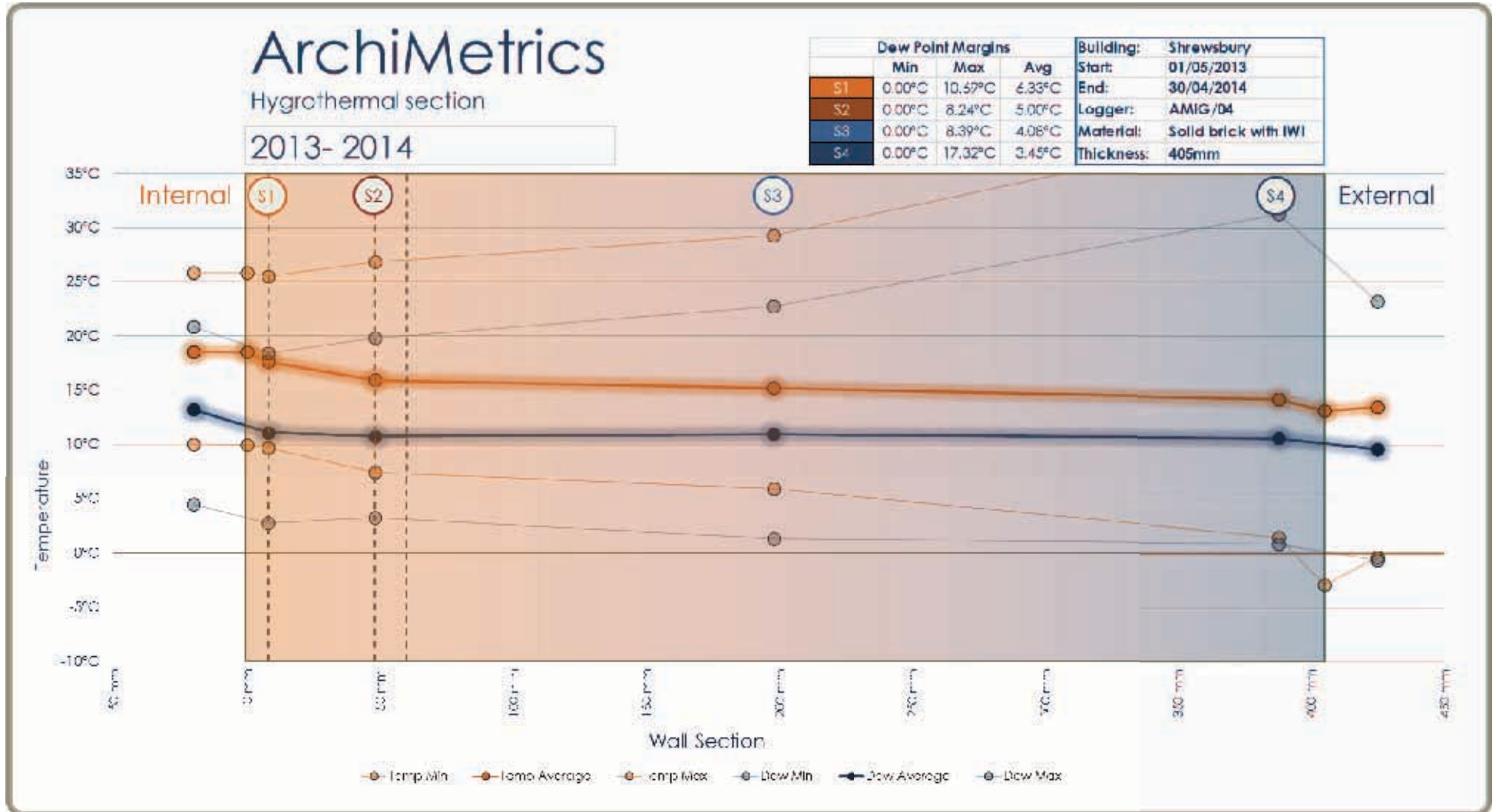
Figure 13. Hygrothermal Section, Abbeyforegate, Shrewsbury, 2013 - 2014.
