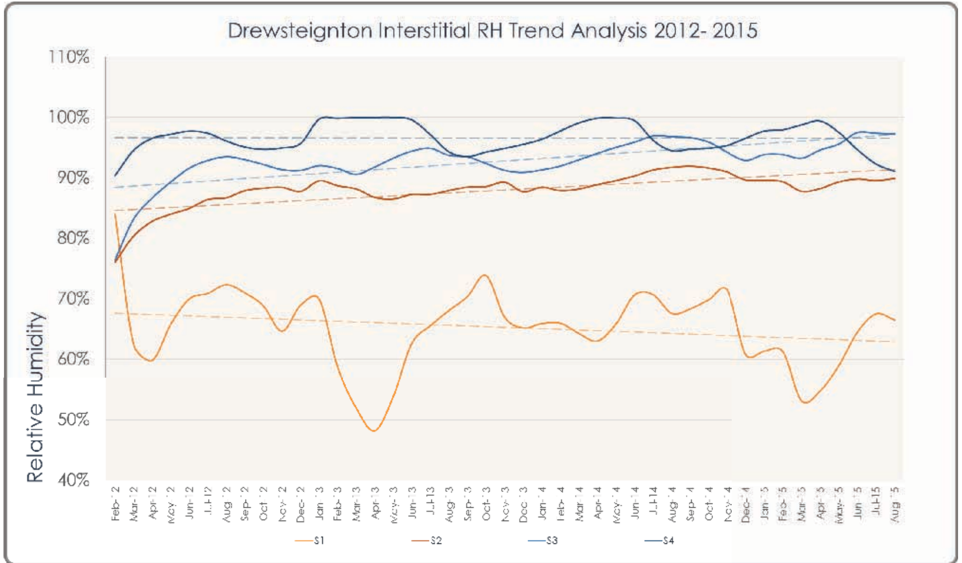
Figure 37: Relative Humidity Trends over time, Drewsteignton 2012 □ 2015.
