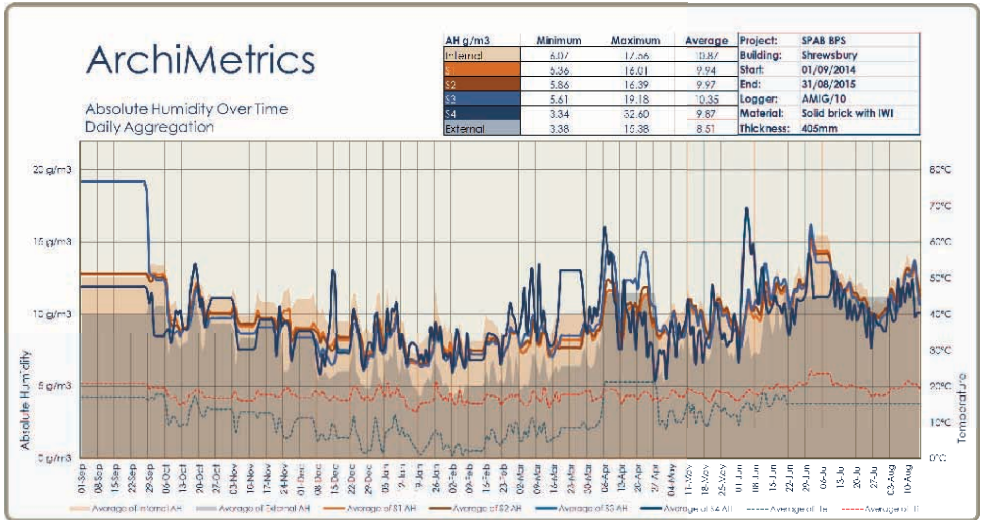
Figure 8: Absolute Humidity over time, Abbeyforegate, Shrewsbury 2014 - 2015.
