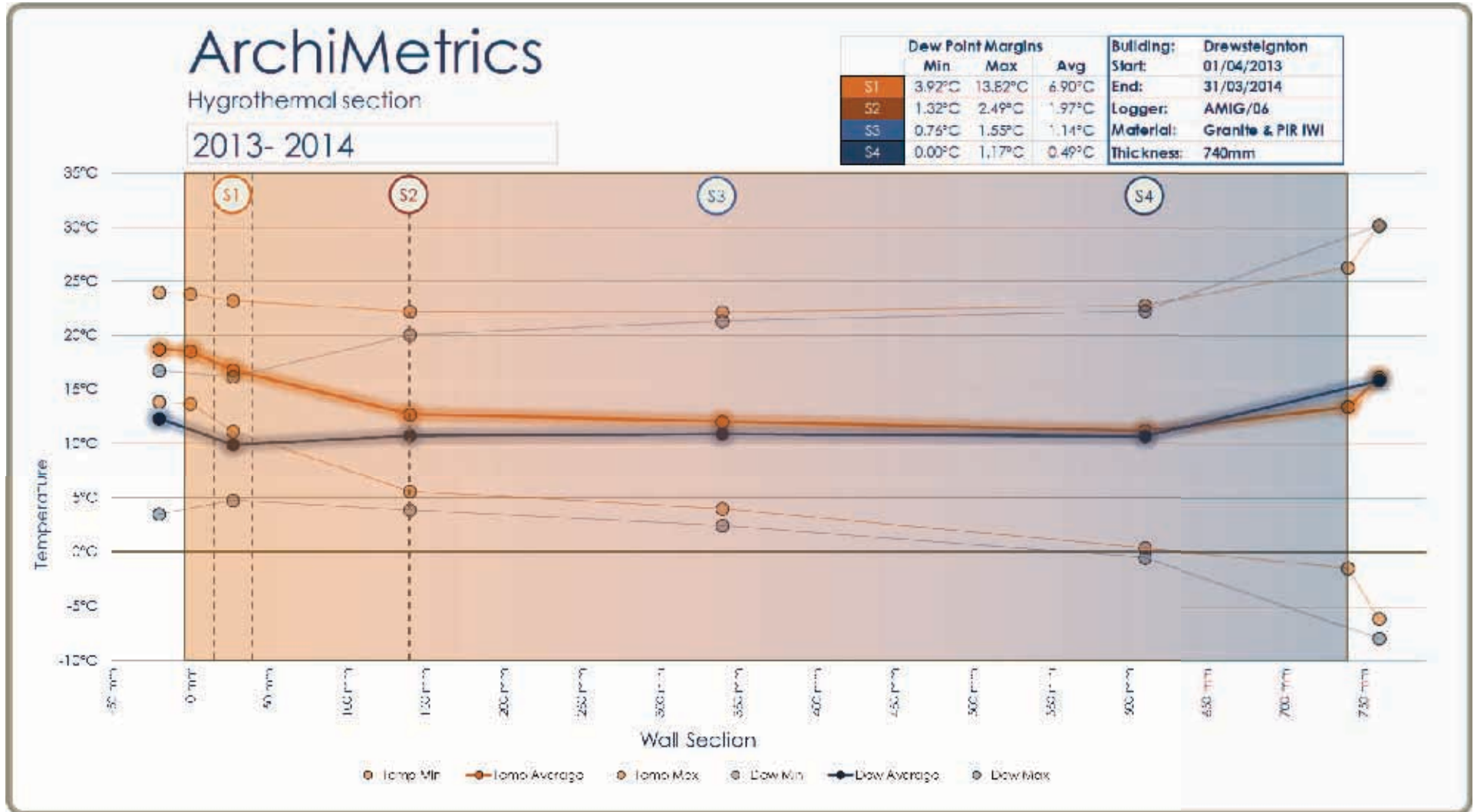
Figure 23. Hygrothermal Section, Mill House, Drewsteignton, 2013 - 2014.
