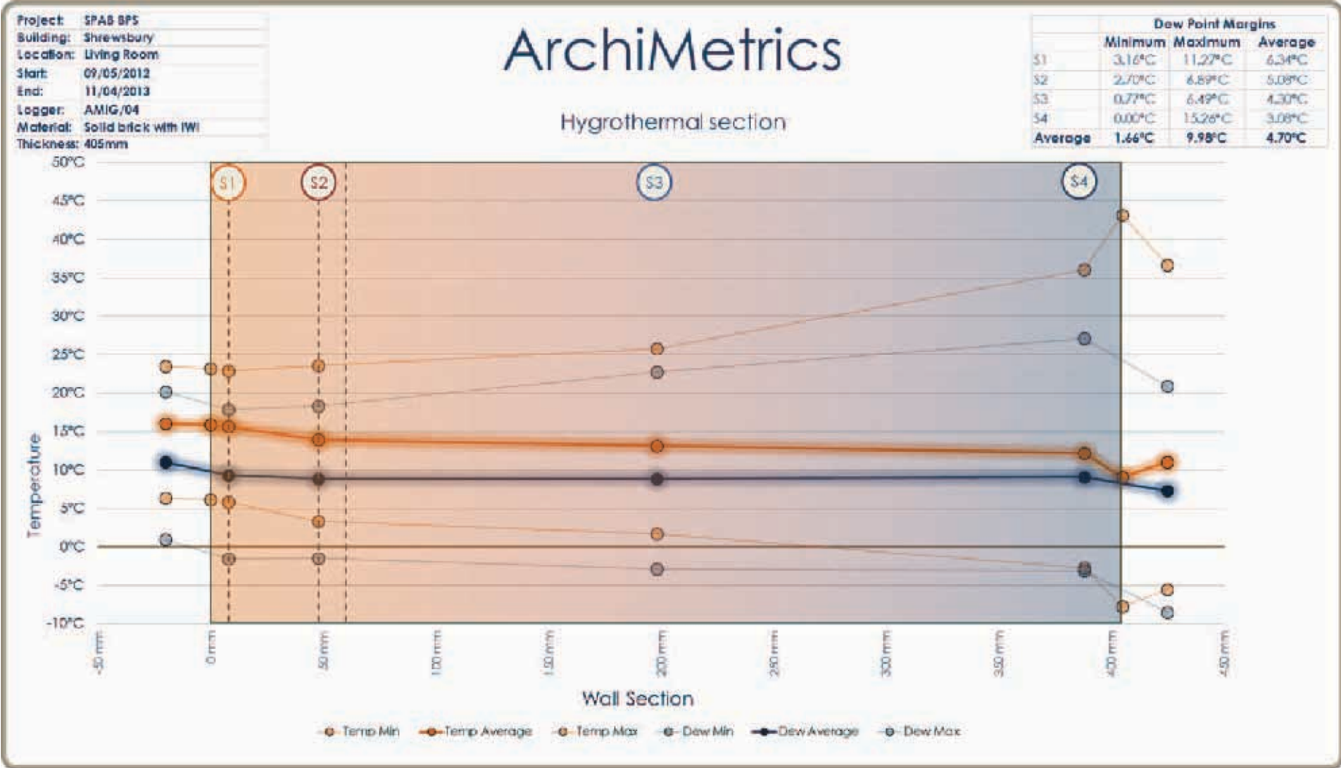
Figure 14. Hygrothermal Section, Abbeyforegate, Shrewsbury, 2012 - 2013.
