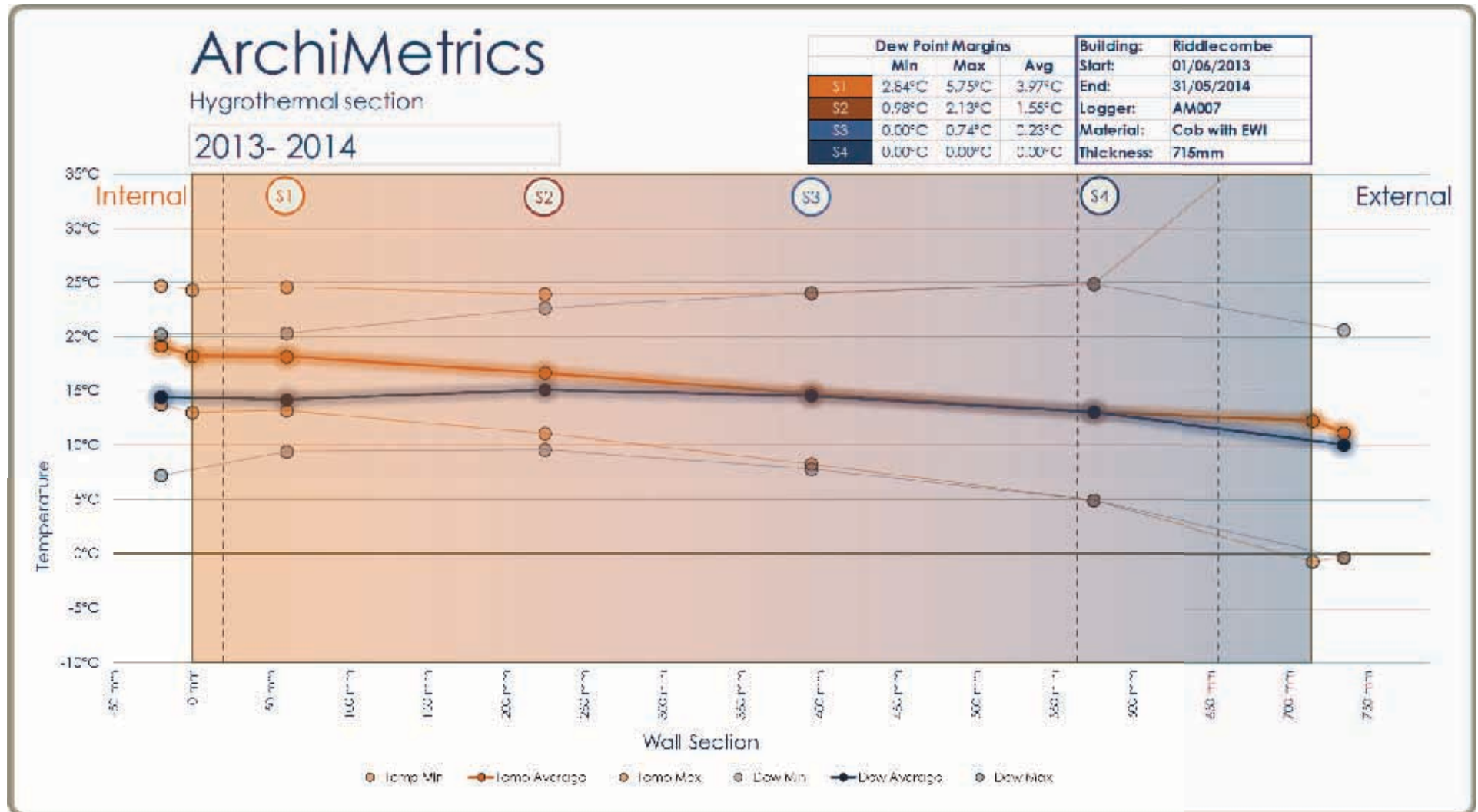
Figure 35. Hygrothermal Section, The Firs, Riddlecombe, 2013 - 2014.
