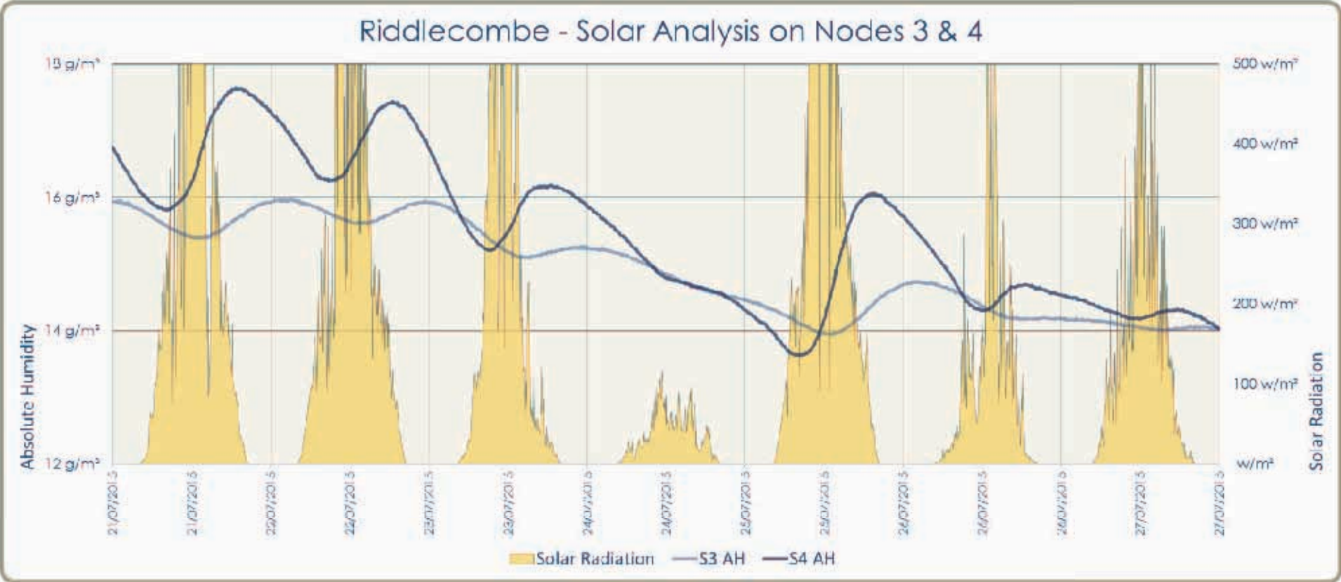
Figure 31: Solar Analysis - Absolute Humidity sensors 3 and 4 over time, Riddlecombe, July 2015.
