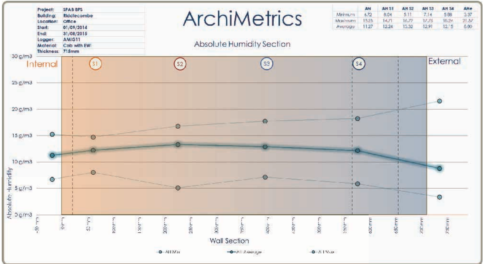
Figure 32: Absolute Humidity average section (capped). Riddlecombe, 2014 □ 2015.
