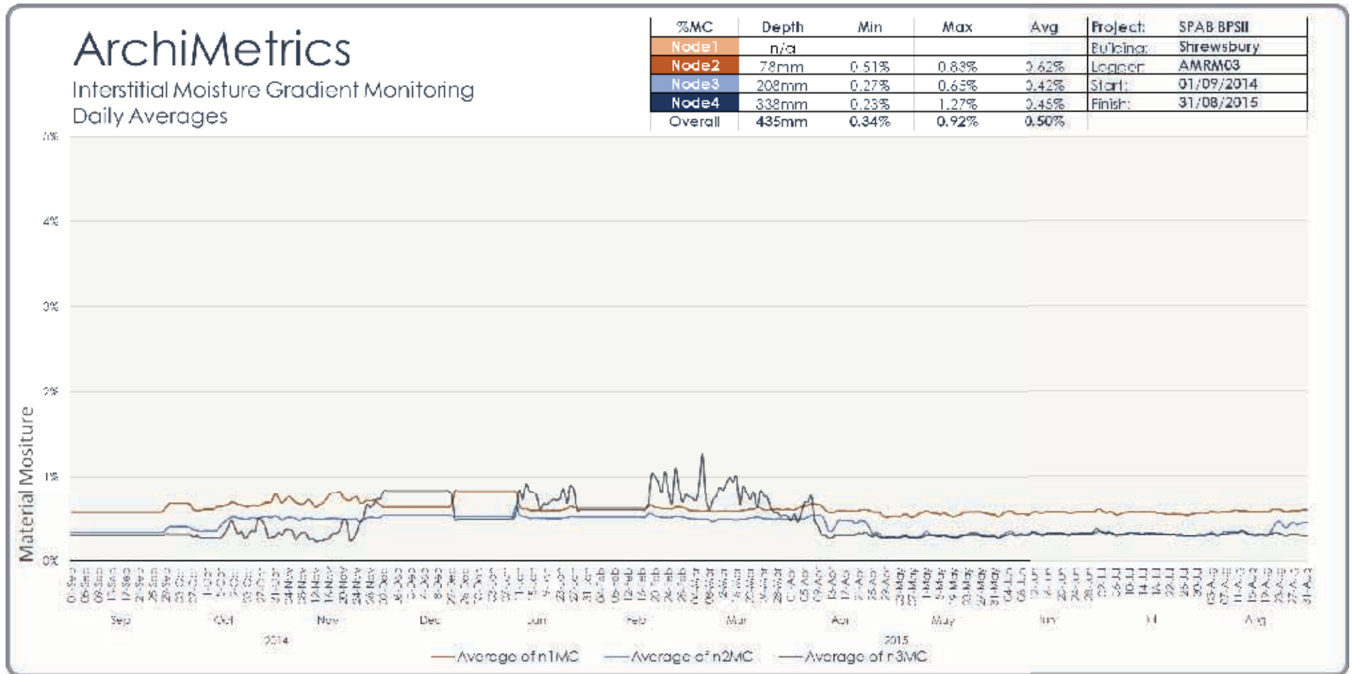
Figure 40: Material moisture content over time, Abbeyforegate, Shrewsbury 2014 - 2015.
