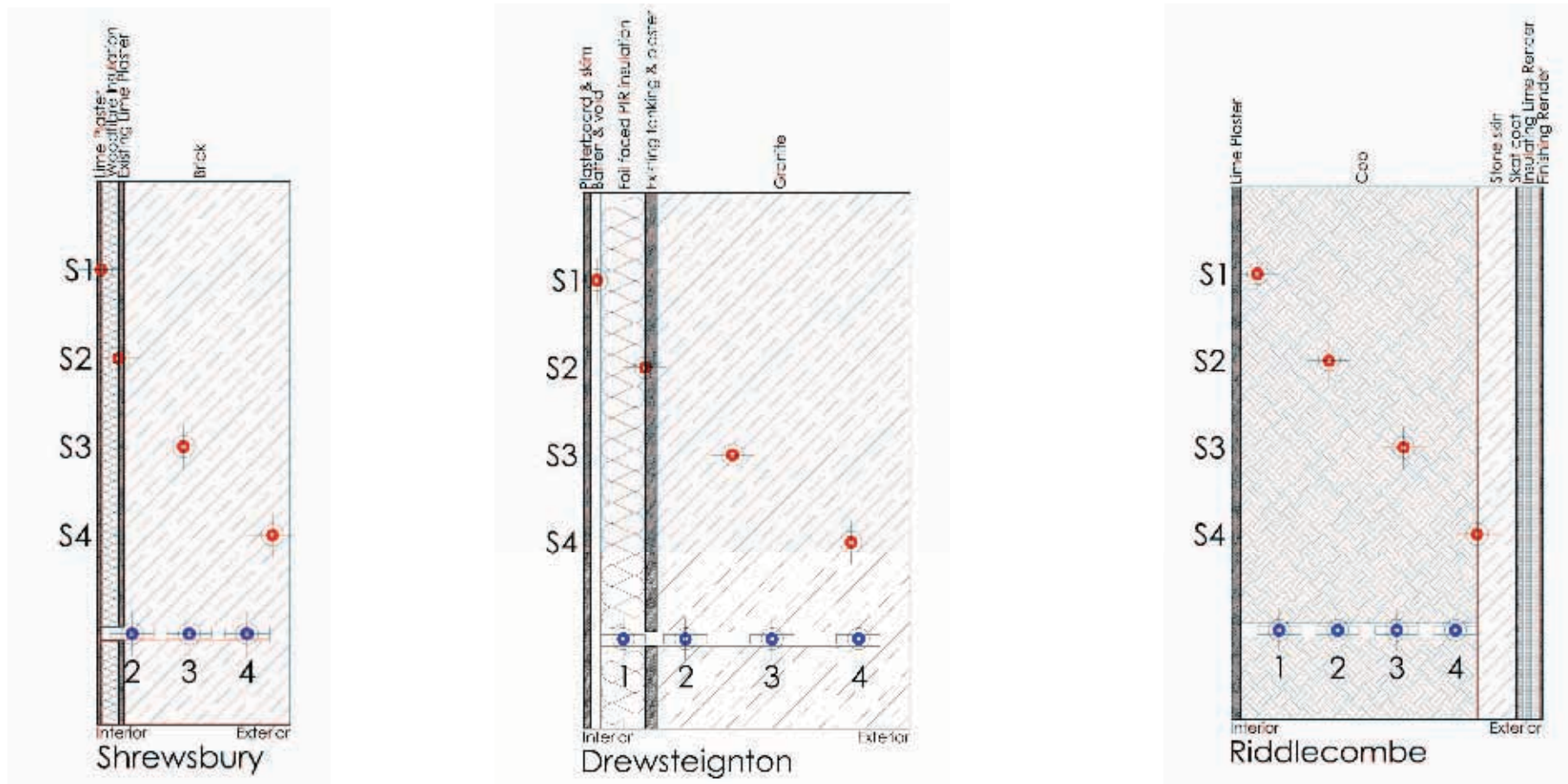
Figure 39. Wall build-ups and sensor positions; IHGM (red) and material moisture (blue).
