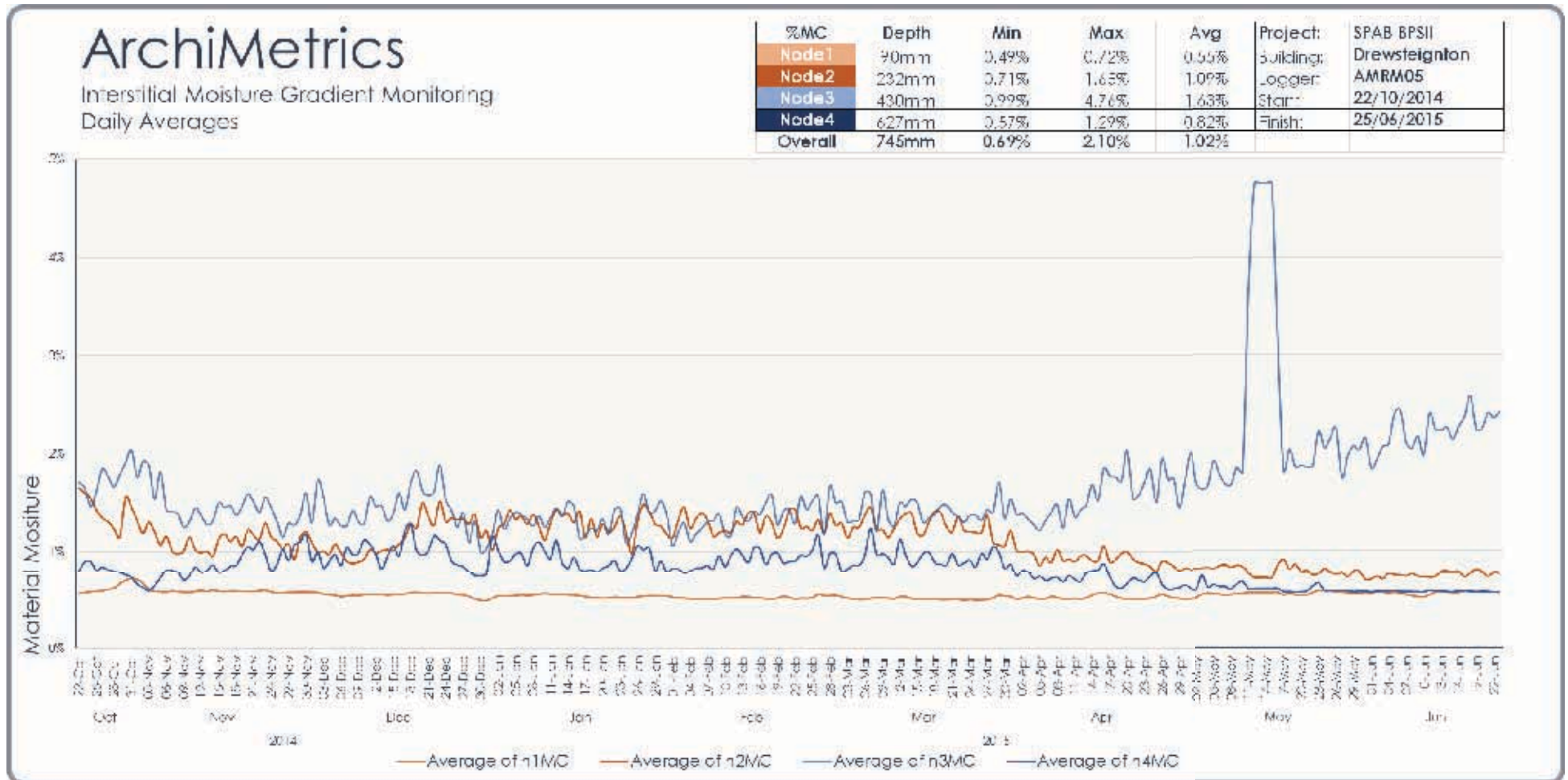
Figure 41: Material moisture content over time, Mill House, Drewsteignton, 2014 - 2015.
