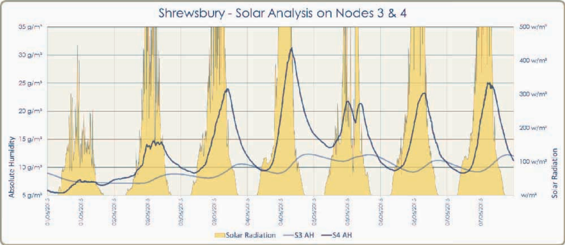
Figure 10: Solar Analysis on nodes 3 and 4 wk. bg. 1 st June 2015, Abbeyforegate, Shrewsbury 2014 - 2015.
