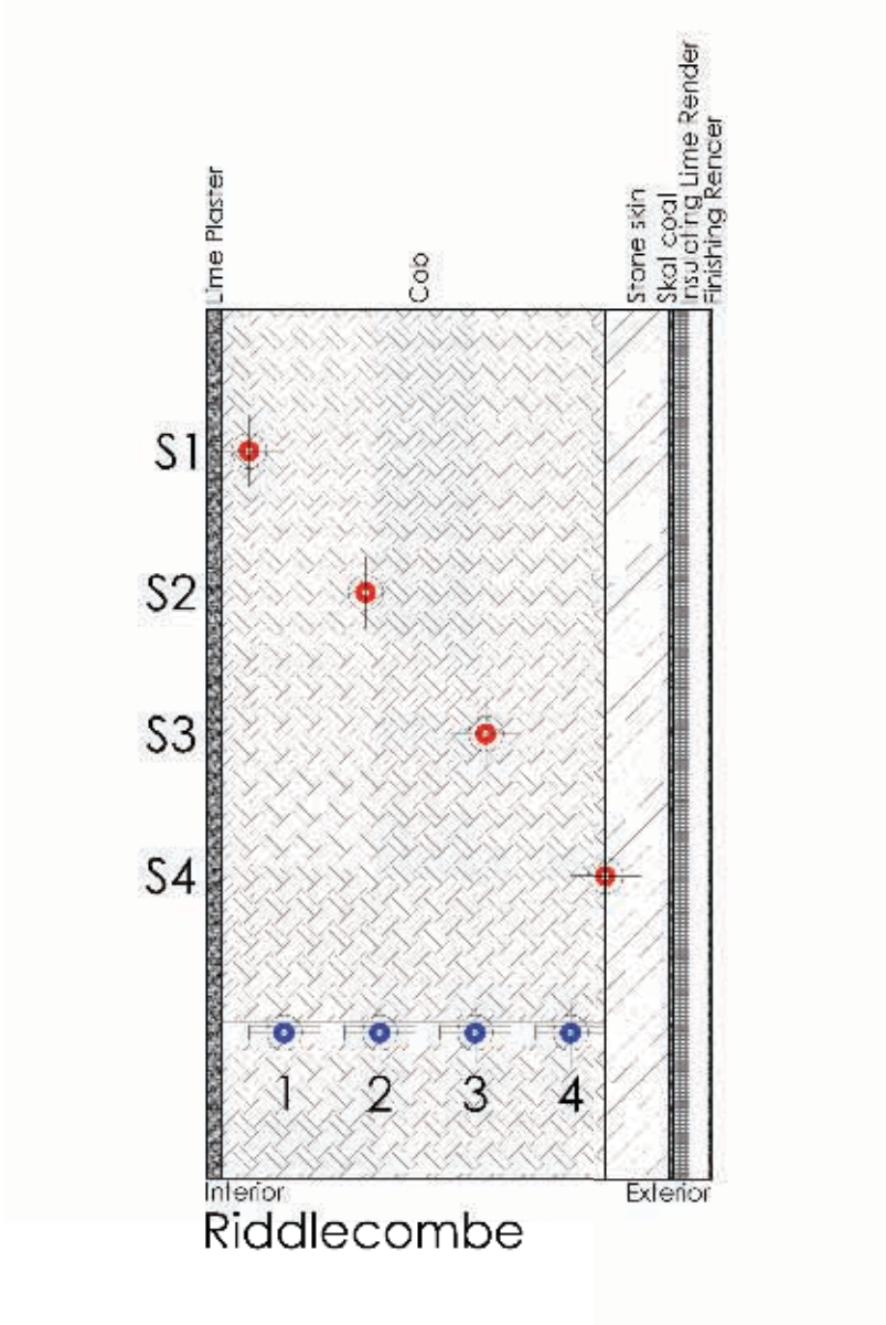
Figure 27. Position of sensors through wall section, Riddlecombe.
