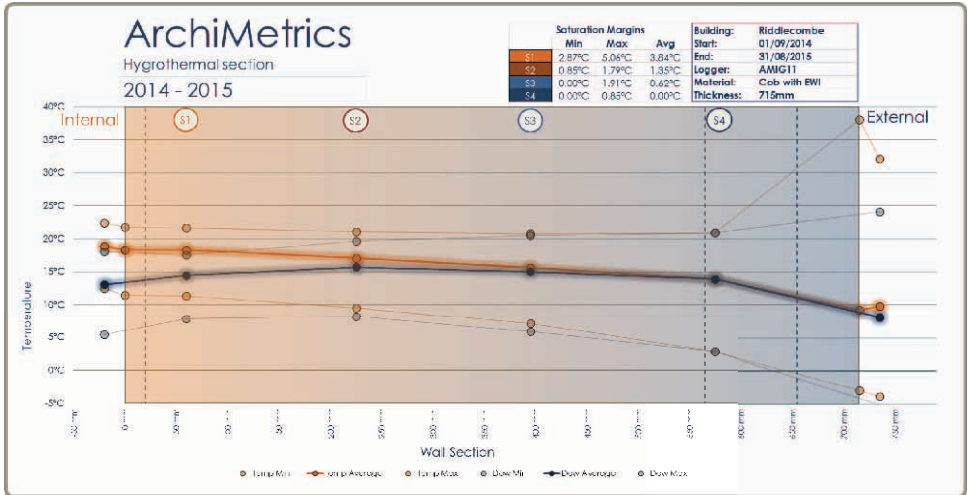
Figure 34. Hygrothermal Section, The Firs, Riddlecombe, 2014 - 2015.
