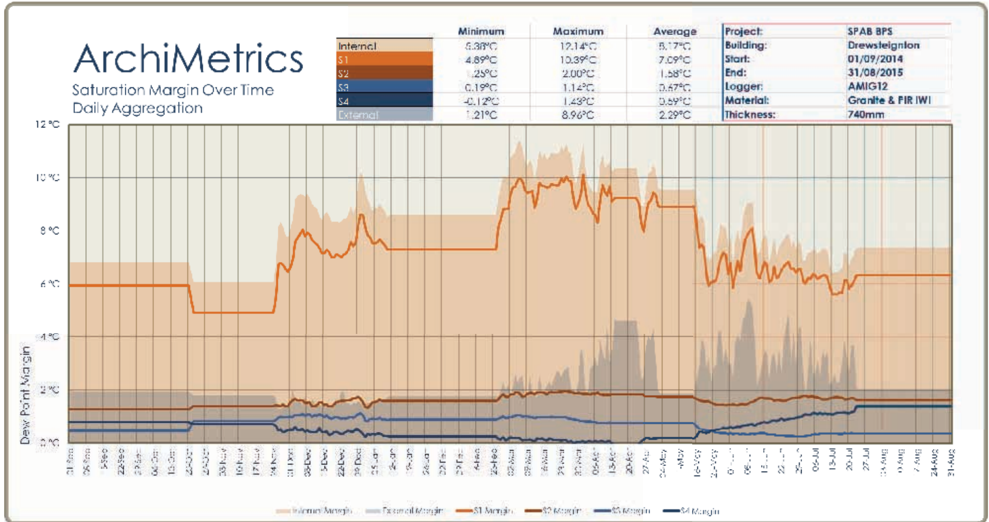
Figure 21. Saturation Margin Over Time, Mill House, Drewsteignton, 2014 - 2015.
