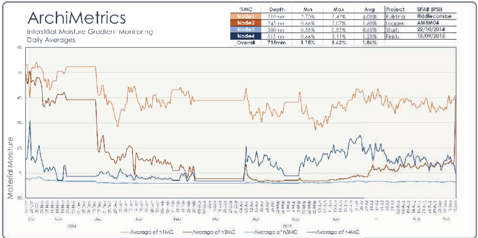
Figure 42: Material moisture content over time, The Firs, Riddlecombe, 2014 - 2015.
