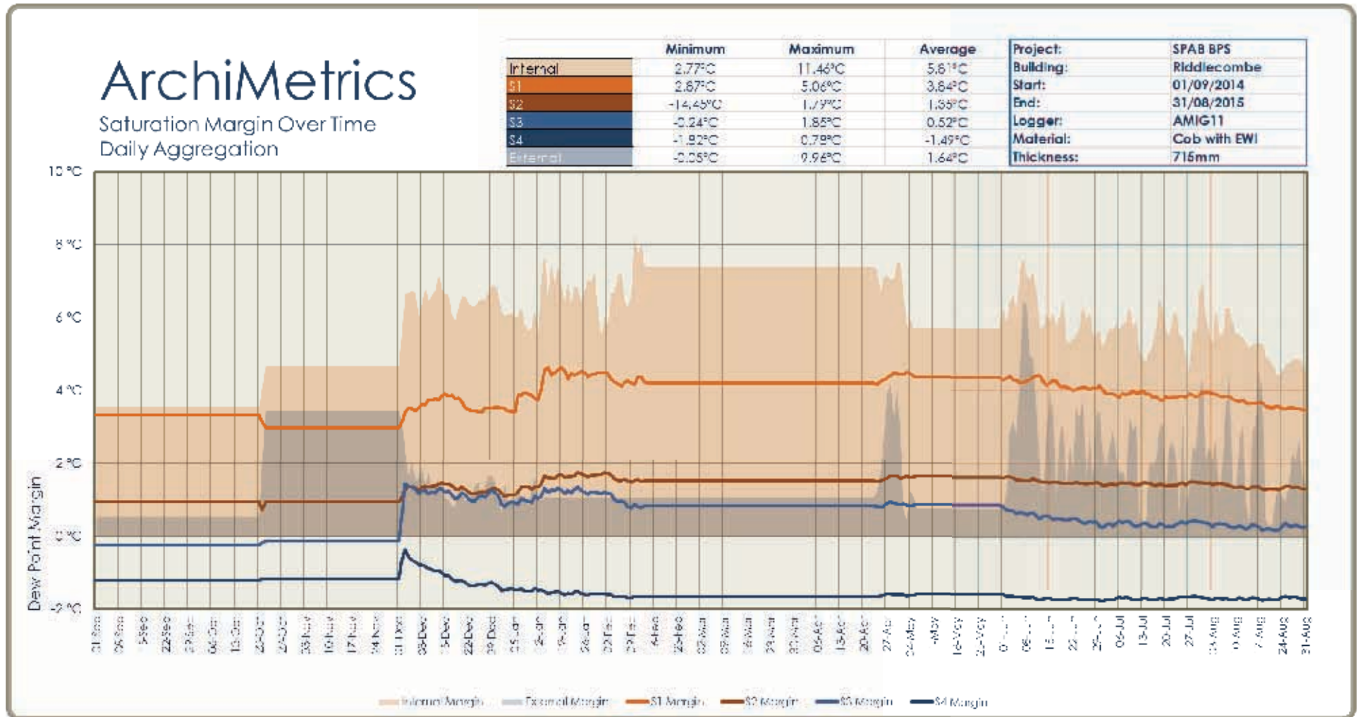
Figure 33. Saturation Margin over time, The Firs, Riddlecombe, 2014 - 2015.
