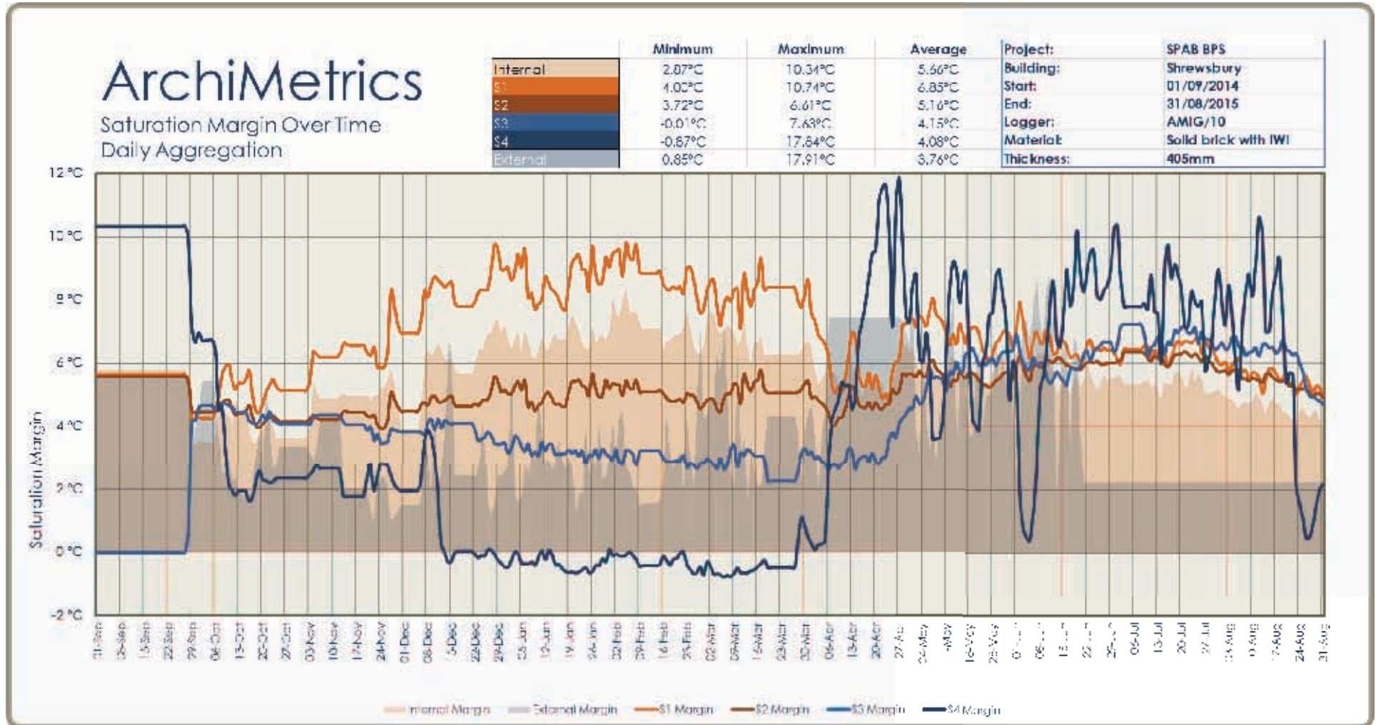
Figure 11. Saturation Margin over time, Abbeyforegate, Shrewsbury 2014 - 2015.
