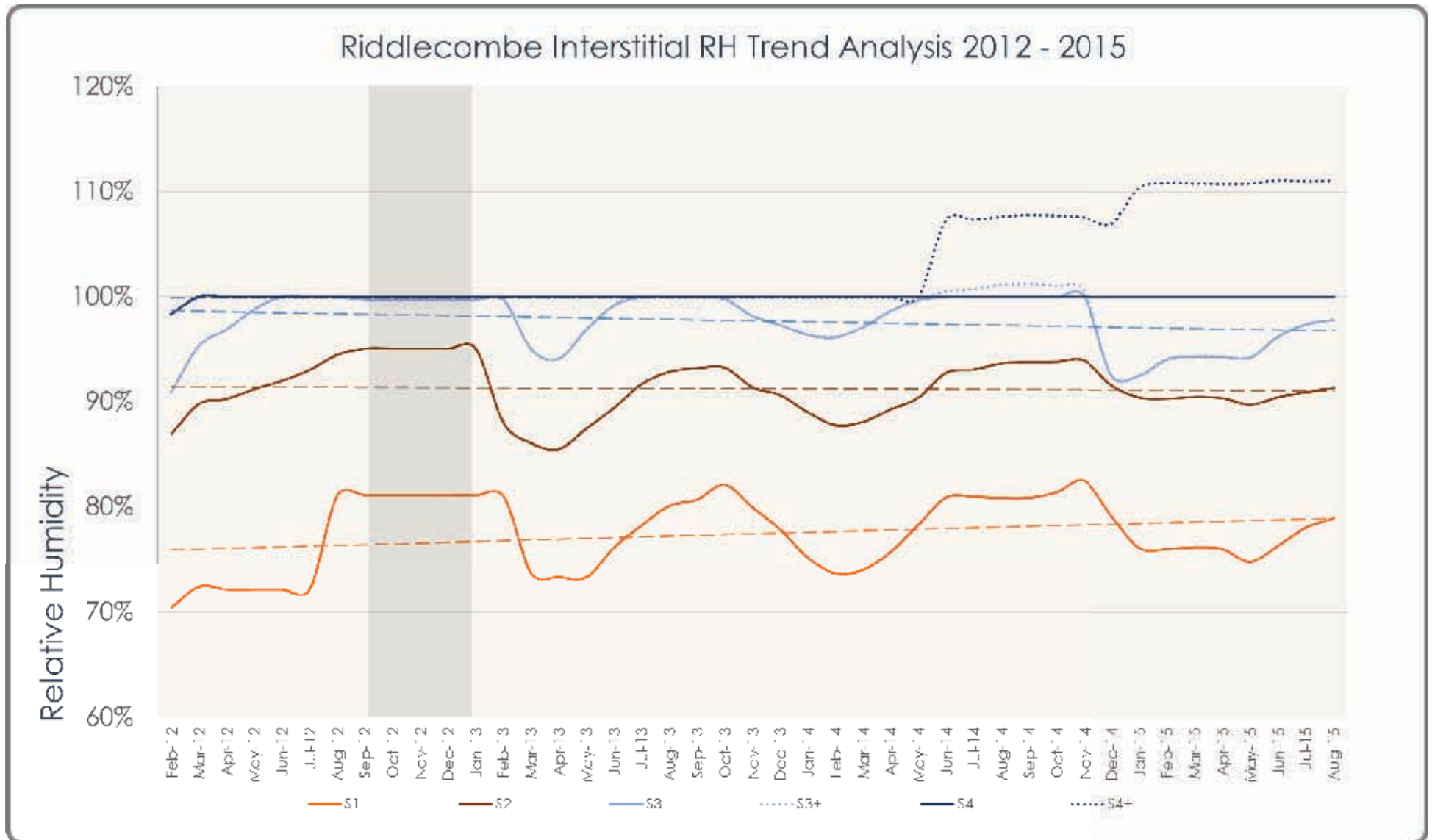
Figure 38. Relative Humidity Trends over time, Riddlecombe, 2012 - 2015.
