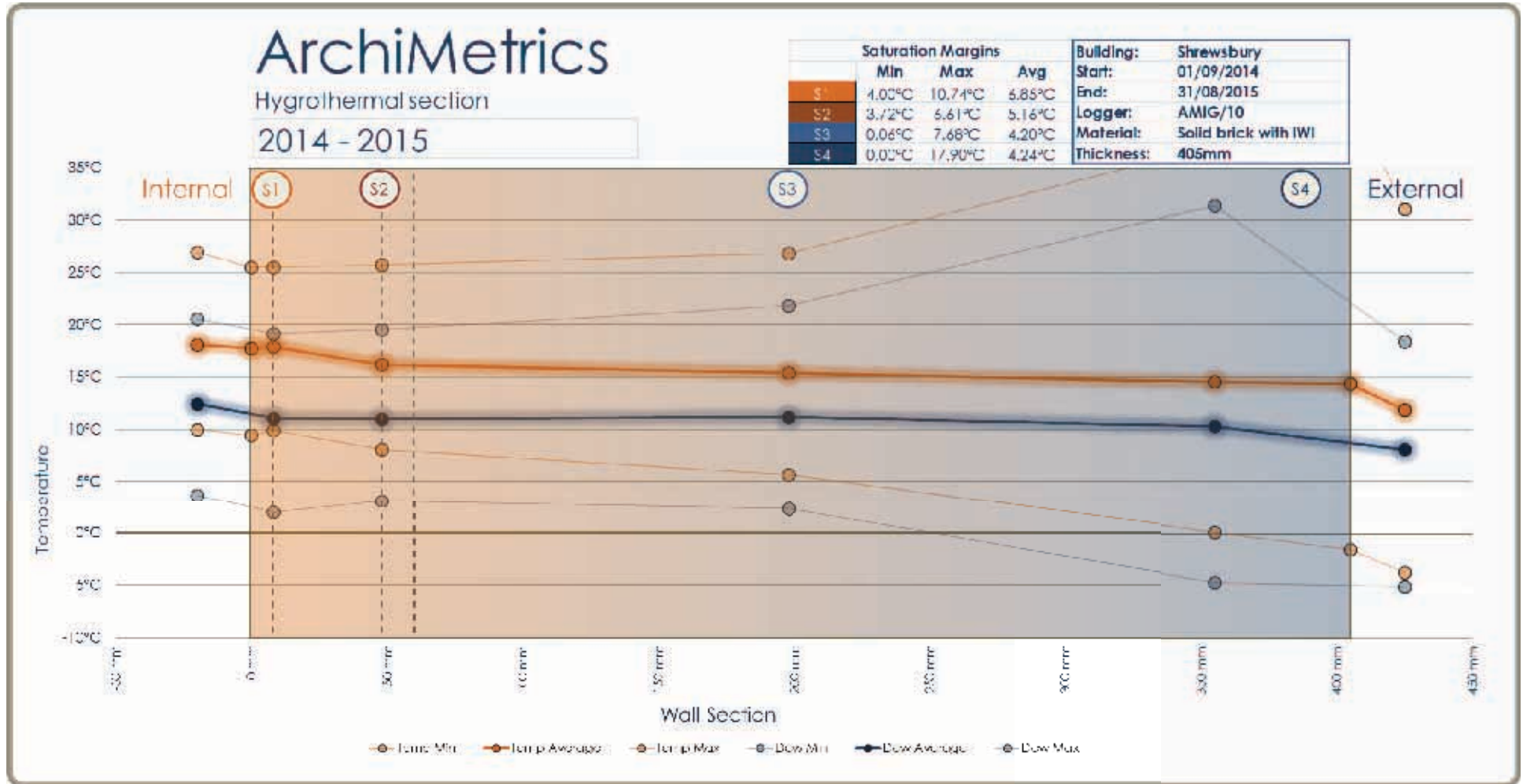
Figure 12. Hygrothermal Section, Abbeyforegate, Shrewsbury 2014 □ 2015 (capped).
