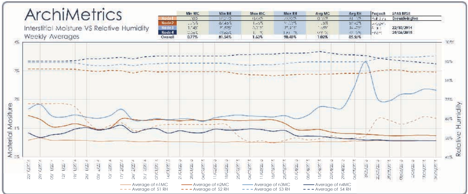
Figure 44. %MC and %RH comparison, Mill House, Drewsteigton, 2014 -15.
