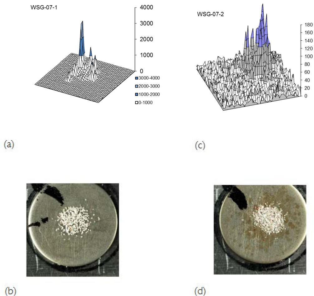
Figure 30: Spatially-resolved OSL (SROSL) from aliquots ( \sim 1\text{--}2 mg) of quartz grains placed on discs of \sim 9.5 mm diameter: isometric views of intensity patterns following the administration of a beta dose where the scan area is \sim 10 \times 10 mm ((a) WSG-07-1, (c) WSG-07-2), and photographic images of the same aliquots showing the distribution of grains on the discs (plan views) ((b) WSG-07-1, (d) WSG-07-2). The SROSL for both WSG-07-1 and WSG-07-2 is heterogenous, and in the case of WSG-07-1 the pattern suggests a small number of very bright grains
