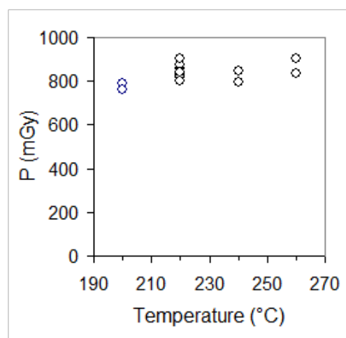
Figure 29: Examples of (a) typical regenerative growth characteristic showing good linearity and (b) a plot of paleodose vs pre-heat temperature
