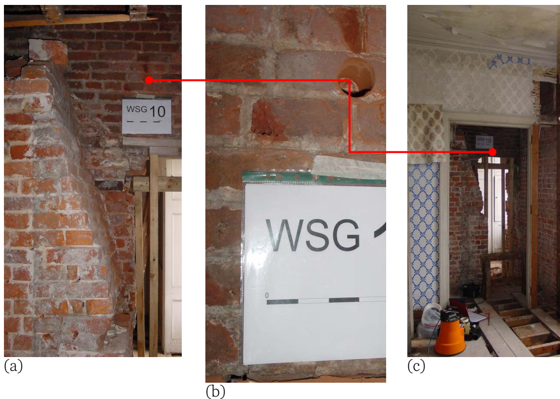
Figure 22: (a) north-facing interior wall on bedchamber floor adjacent to chimney stack in the Southampton Room, showing location of WSG-10, (b) close-up of sampling location WSG-10, (c) general view of location of WSG-10 in relation to west-facing exterior wall
