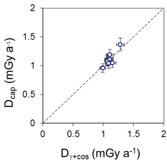
Figure 31: Comparison of the values of the combined gamma and cosmic annual dose at locations 1–9, obtained directly using dosemeters ( D_{\text{cap}} ) and indirectly ( D_{\gamma+\cos} ) based on measurements of brick radioactivity, as discussed in the text. The line plotted represents a line of concordance
