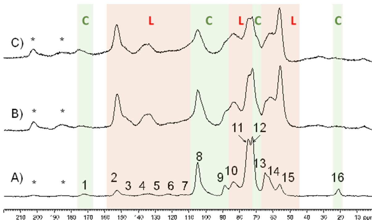
Figure 14: Examples of typical CP-MAS ^{13}\text{C} high-resolution solid-state NMR spectra of modern beech (A) and archaeological beech samples with water contents of 82% (B) and 91% (C). Peaks highlighted in green relate to the carbohydrate components (C) and those in red relate to lignin (L) (a full assignment can be found in Bardet et al., 2002). An increase in relative intensity of the lignin compared to carbohydrate peaks is observed in the archaeological samples. Signal 16 relates to \text{CH}_3 groups in hemicellulose and is completely absent in the archaeological samples. Signal 2 relates to \beta\text{-O-4} linkages and is retained in all samples. Adapted from Bardet et al., 2002 with permission from American Chemical Society, copyright 2002.
