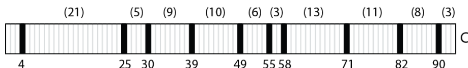
Figure 10: Schematic illustration of sample b&t08 to locate the single-ring sub-samples submitted for radiocarbon dating. C = bark edge, winter felled
