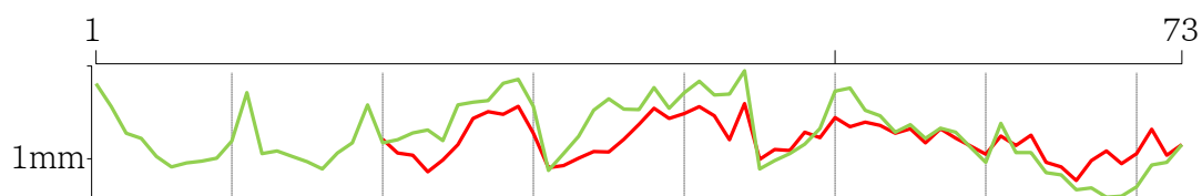
Figure 5: Plots of b&t05 (red; relative years 20–73) and b&t06 (green; relative years 1–73) showing their similarity in growth. The y-axis is ring width on a logarithmic scale
