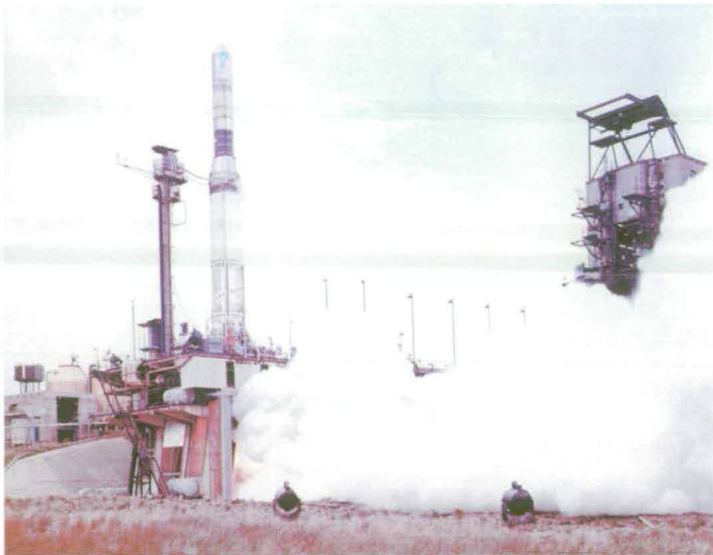
Figure 356 Missile Test Stand C3 was illuminated by mobile searchlights on wooden rails some distance from the stand © Rolls-Royce plc
