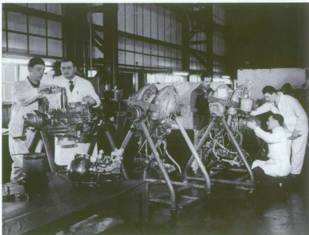
Figure 15 Work on Blue Streak rocket engines was relocated from Derby to building F1 at Spadeadam © Rolls-Royce plc
