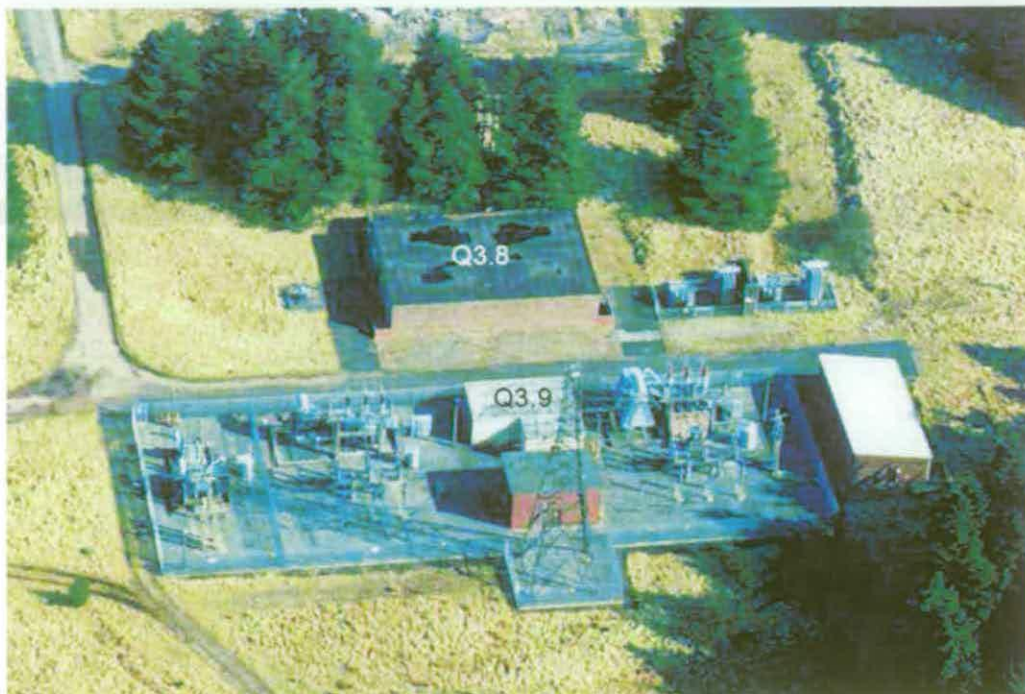
Figure 92 Modern aerial photograph of the Central Electricity Generating Board Compound Q3 © English Heritage NMR (17818/05)
