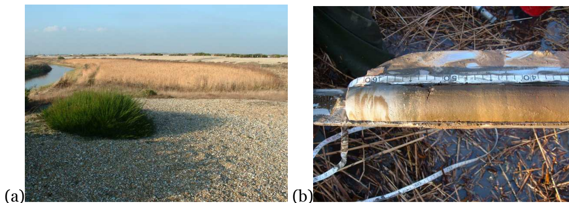
Figure 26. Muddymore Pit, Dungeness Foreland, Kent: (a) general site view and (b) core section showing the sediments changing from the clastic basal sediments (left) to the overlying organic sediments (right). Photos: © Martyn Waller.
