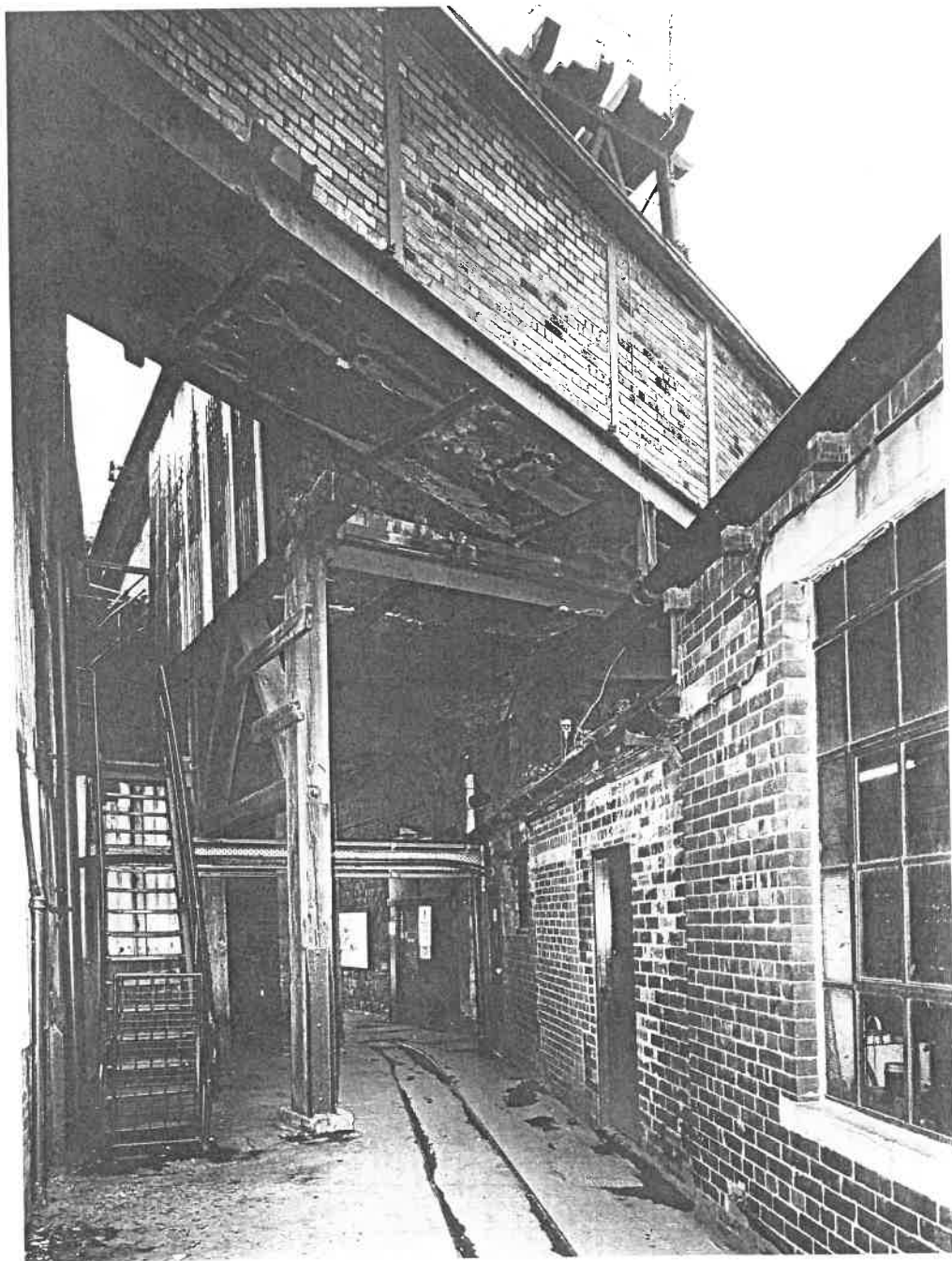
Fig 15 Caphouse Pit. Detail of timber support for walkway on north-west side of heapstead over No. 1 Shaft. Screens building to left, workshops to right. RCHME AA97/4952.
