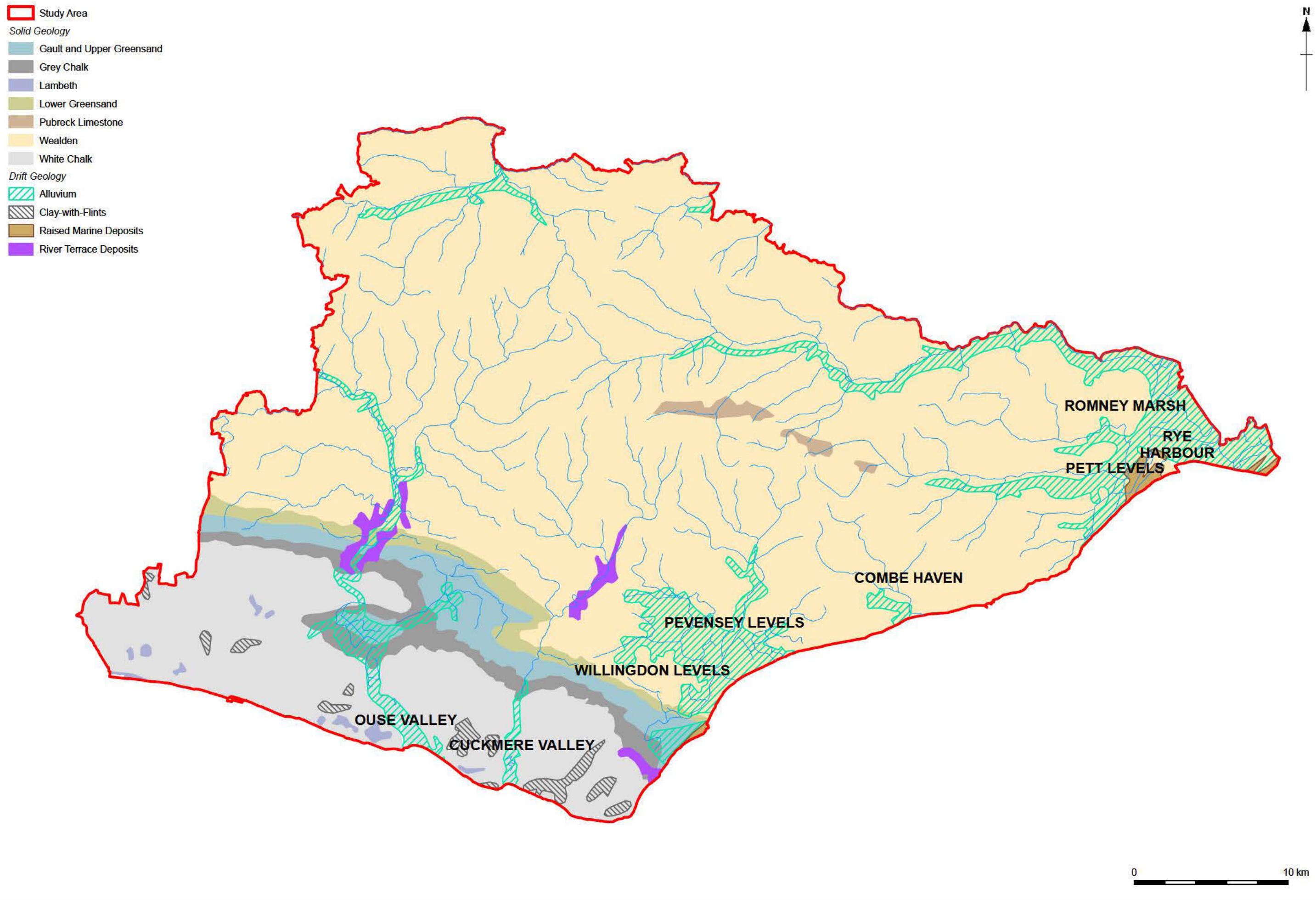
Figure 3: Solid and drift geology of East Sussex
