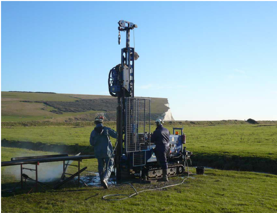
Plate 4: Borehole sampling within the Cuckmere Haven, East Sussex
